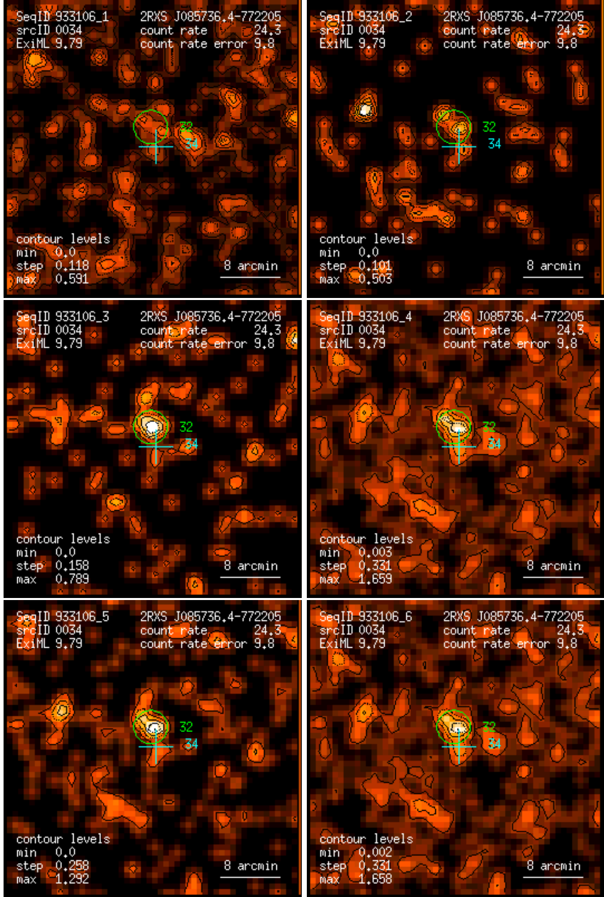
Figure 34: RASS 933106: detection 0034: band rate images, Gaussian filter: (1) PSPC channels 11 – 41, (2) 52 – 90, (3) 91 – 201, (4) 11 – 235, (5) 52 – 201, (6) 11 – 201. Broad band rates in counts/ks. Band rate contour levels in counts/ks/arcmin 2 .
