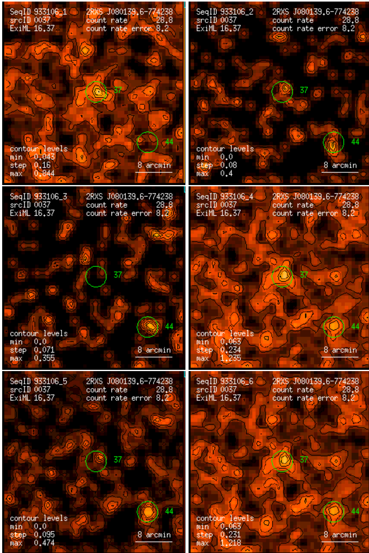
Figure 37: RASS 933106: detection 0037: band rate images, Gaussian filter: (1) PSPC channels 11 – 41, (2) 52 – 90, (3) 91 – 201, (4) 11 – 235, (5) 52 – 201, (6) 11 – 201. Broad band rates in counts/ks. Band rate contour levels in counts/ks/arcmin 2 .
