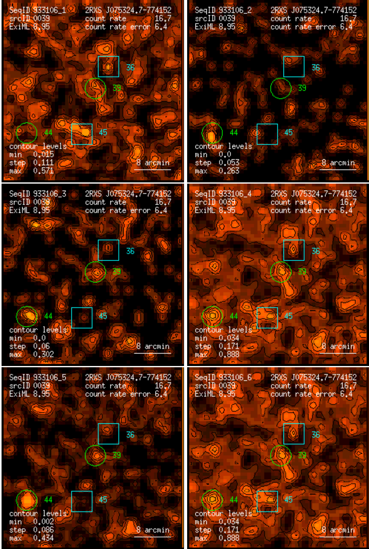
Figure 39: RASS 933106: detection 0039: band rate images, Gaussian filter: (1) PSPC channels 11 – 41, (2) 52 – 90, (3) 91 – 201, (4) 11 – 235, (5) 52 – 201, (6) 11 – 201. Broad band rates in counts/ks. Band rate contour levels in counts/ks/arcmin 2 .
