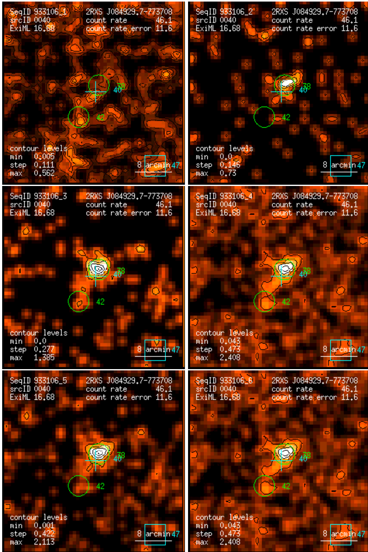
Figure 40: RASS 933106: detection 0040: band rate images, Gaussian filter: (1) PSPC channels 11 – 41, (2) 52 – 90, (3) 91 – 201, (4) 11 – 235, (5) 52 – 201, (6) 11 – 201. Broad band rates in counts/ks. Band rate contour levels in counts/ks/arcmin 2 .
