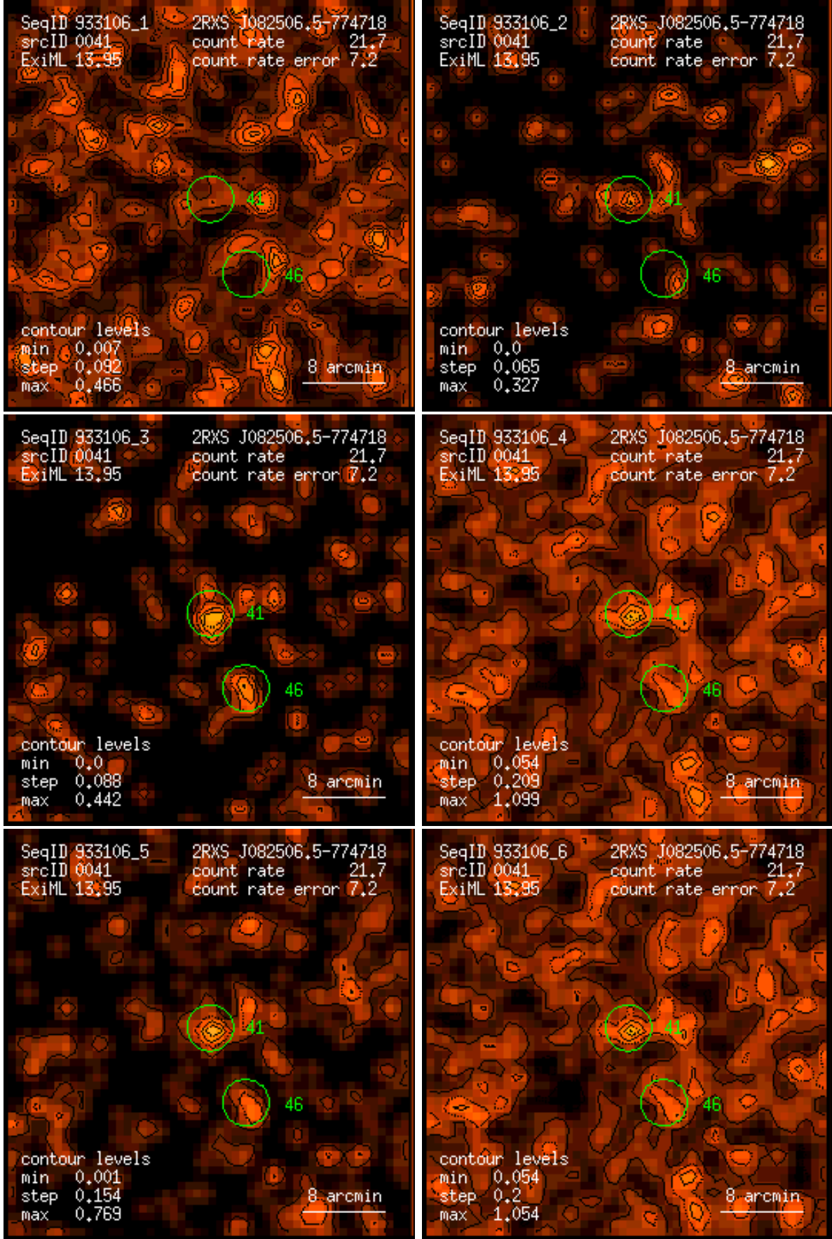
Figure 41: RASS 933106: detection 0041: band rate images, Gaussian filter: (1) PSPC channels 11 – 41, (2) 52 – 90, (3) 91 – 201, (4) 11 – 235, (5) 52 – 201, (6) 11 – 201. Broad band rates in counts/ks. Band rate contour levels in counts/ks/arcmin 2 .
