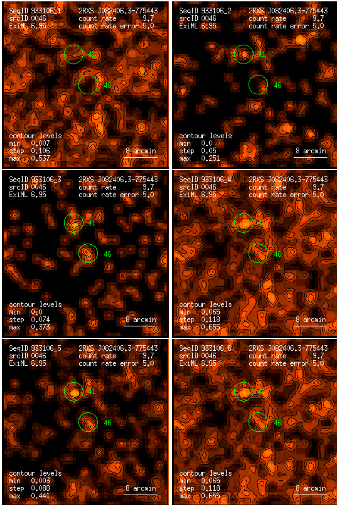
Figure 46: RASS 933106: detection 0046: band rate images, Gaussian filter: (1) PSPC channels 11 – 41, (2) 52 – 90, (3) 91 – 201, (4) 11 – 235, (5) 52 – 201, (6) 11 – 201. Broad band rates in counts/ks. Band rate contour levels in counts/ks/arcmin 2 .
