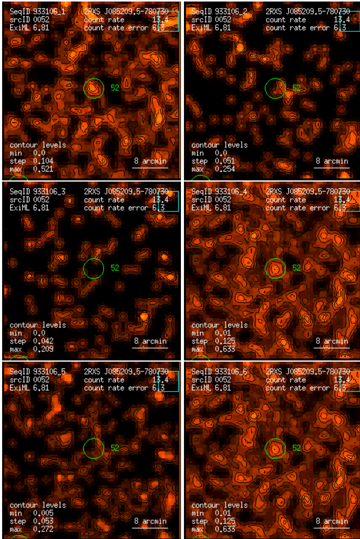
Figure 52: RASS 933106: detection 0052: band rate images, Gaussian filter: (1) PSPC channels 11 – 41, (2) 52 – 90, (3) 91 – 201, (4) 11 – 235, (5) 52 – 201, (6) 11 – 201. Broad band rates in counts/ks. Band rate contour levels in counts/ks/arcmin 2 .
