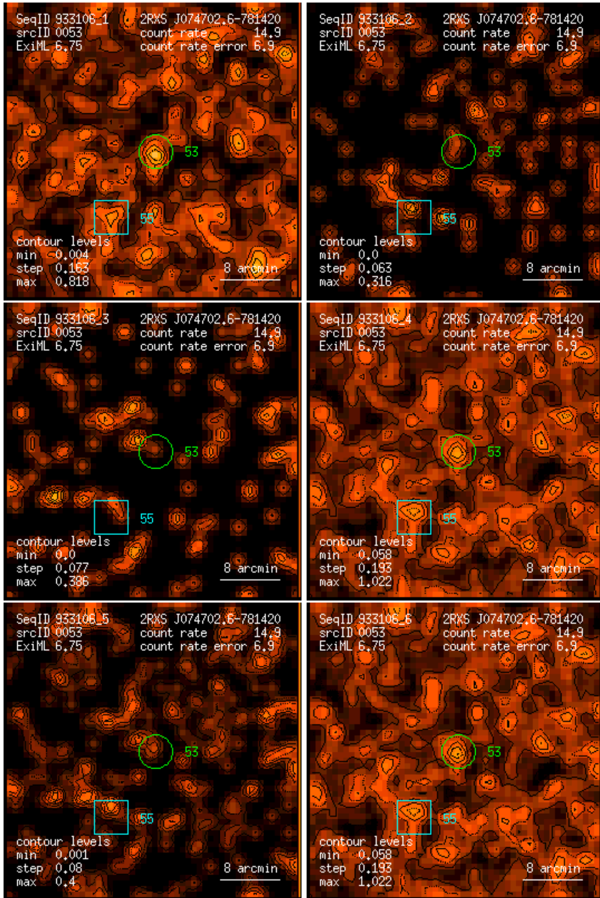
Figure 53: RASS 933106: detection 0053: band rate images, Gaussian filter: (1) PSPC channels 11 – 41, (2) 52 – 90, (3) 91 – 201, (4) 11 – 235, (5) 52 – 201, (6) 11 – 201. Broad band rates in counts/ks. Band rate contour levels in counts/ks/arcmin 2 .
