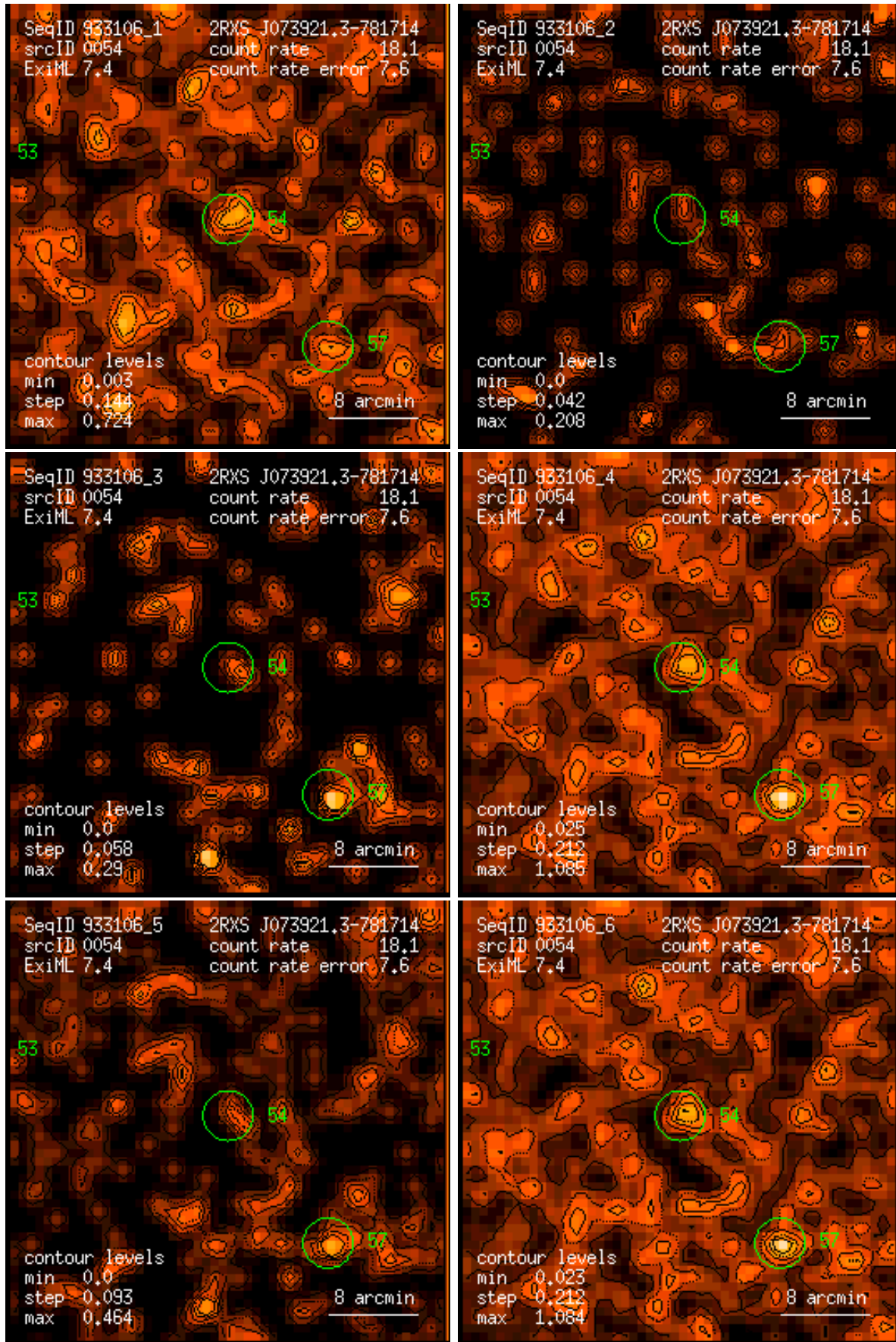
Figure 54: RASS 933106: detection 0054: band rate images, Gaussian filter: (1) PSPC channels 11 – 41, (2) 52 – 90, (3) 91 – 201, (4) 11 – 235, (5) 52 – 201, (6) 11 – 201. Broad band rates in counts/ks. Band rate contour levels in counts/ks/arcmin 2 .
