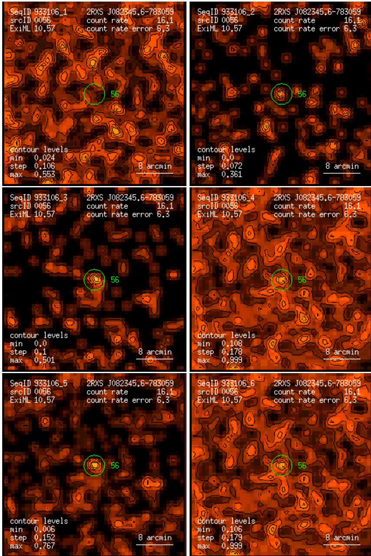
Figure 56: RASS 933106: detection 0056: band rate images, Gaussian filter: (1) PSPC channels 11 – 41, (2) 52 – 90, (3) 91 – 201, (4) 11 – 235, (5) 52 – 201, (6) 11 – 201. Broad band rates in counts/ks. Band rate contour levels in counts/ks/arcmin 2 .
