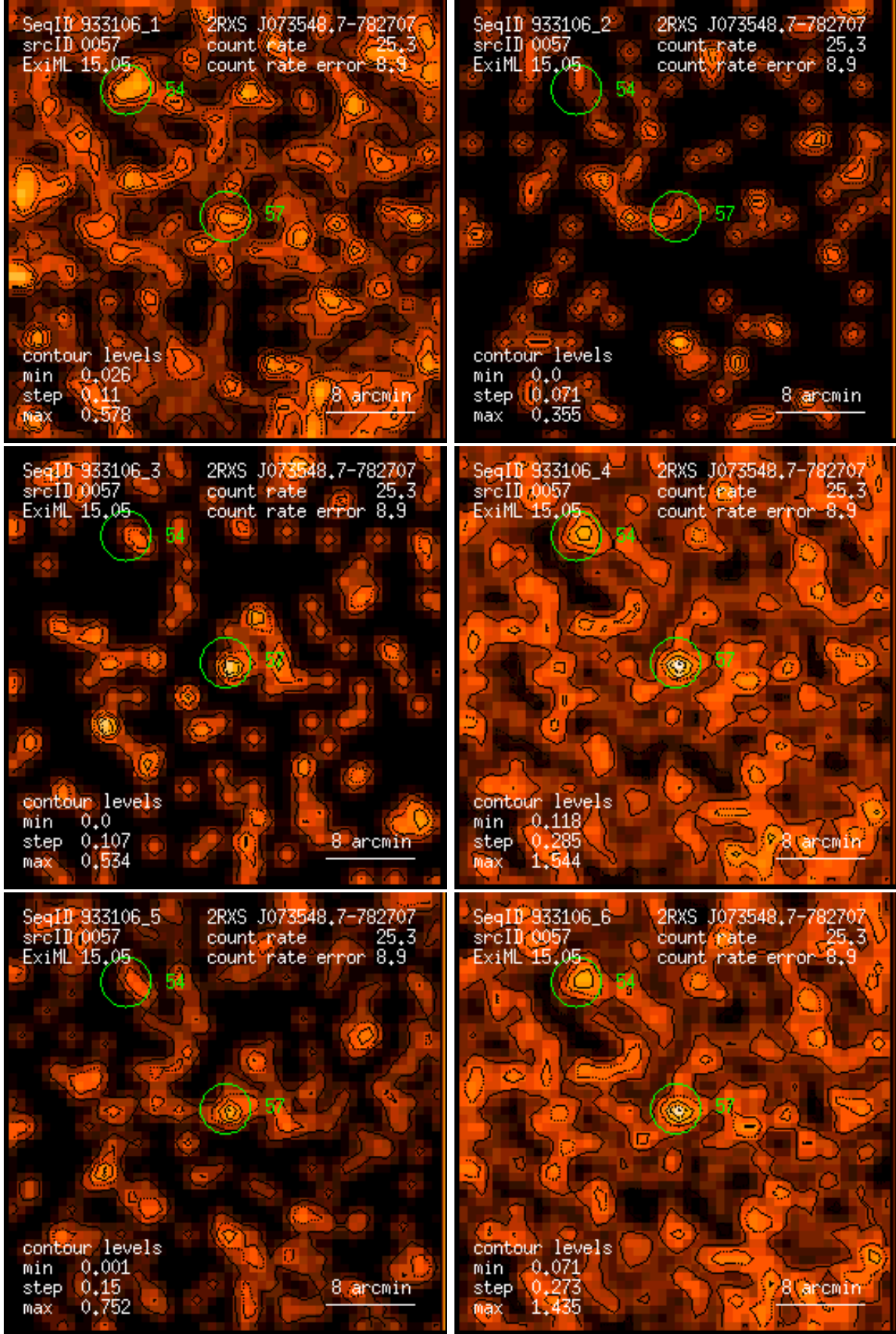
Figure 57: RASS 933106: detection 0057: band rate images, Gaussian filter: (1) PSPC channels 11 – 41, (2) 52 – 90, (3) 91 – 201, (4) 11 – 235, (5) 52 – 201, (6) 11 – 201. Broad band rates in counts/ks. Band rate contour levels in counts/ks/arcmin 2 .
