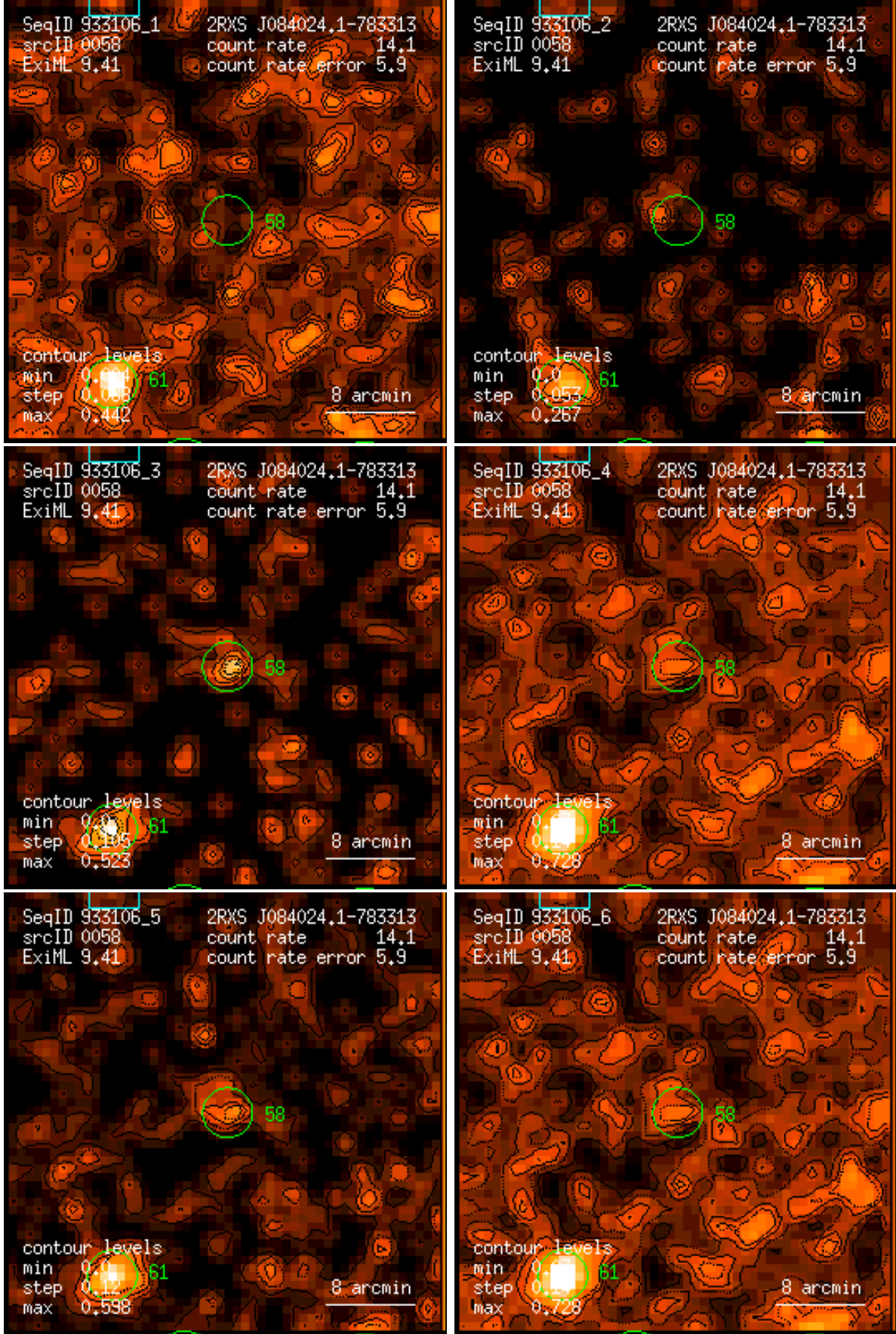
Figure 58: RASS 933106: detection 0058: band rate images, Gaussian filter: (1) PSPC channels 11 – 41, (2) 52 – 90, (3) 91 – 201, (4) 11 – 235, (5) 52 – 201, (6) 11 – 201. Broad band rates in counts/ks. Band rate contour levels in counts/ks/arcmin 2 .
