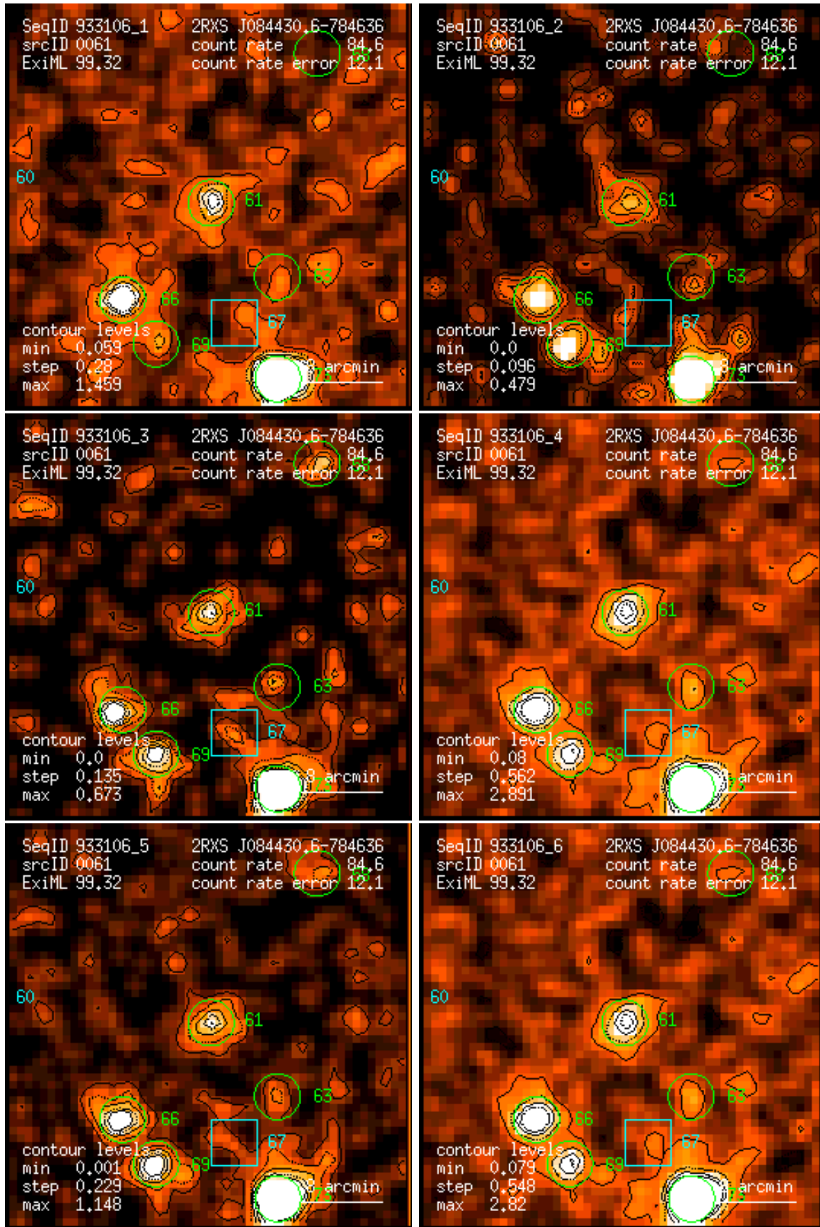
Figure 61: RASS 933106: detection 0061: band rate images, Gaussian filter: (1) PSPC channels 11 – 41, (2) 52 – 90, (3) 91 – 201, (4) 11 – 235, (5) 52 – 201, (6) 11 – 201. Broad band rates in counts/ks. Band rate contour levels in counts/ks/arcmin 2 .
