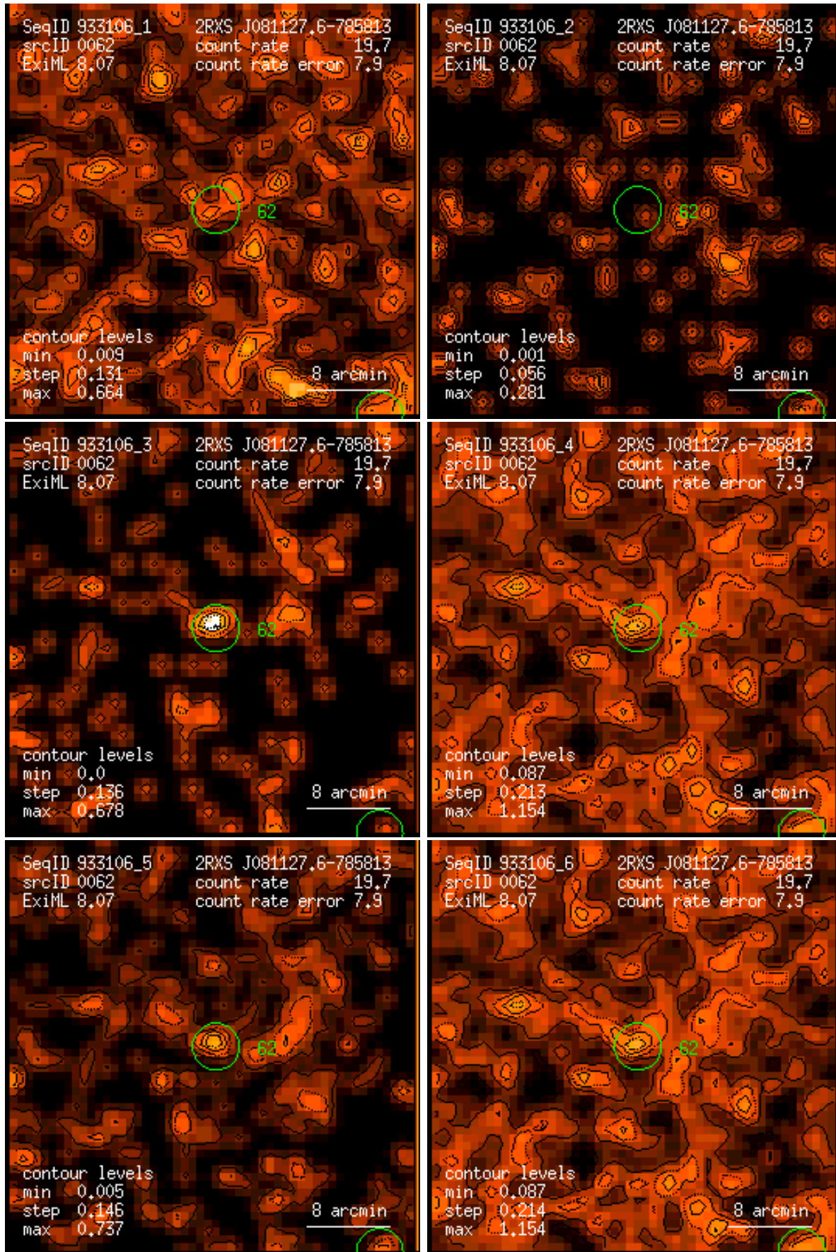
Figure 62: RASS 933106: detection 0062: band rate images, Gaussian filter: (1) PSPC channels 11 – 41, (2) 52 – 90, (3) 91 – 201, (4) 11 – 235, (5) 52 – 201, (6) 11 – 201. Broad band rates in counts/ks. Band rate contour levels in counts/ks/arcmin 2 .
