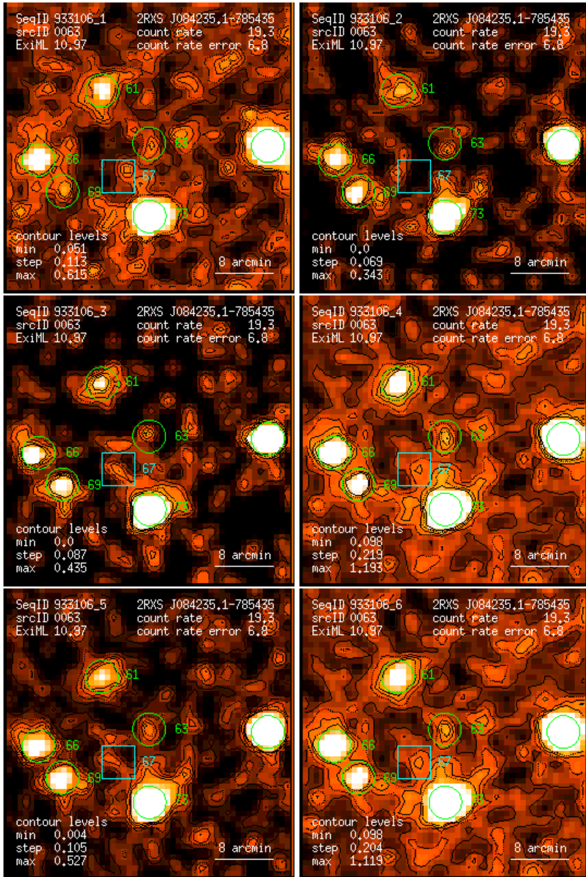
Figure 63: RASS 933106: detection 0063: band rate images, Gaussian filter: (1) PSPC channels 11 – 41, (2) 52 – 90, (3) 91 – 201, (4) 11 – 235, (5) 52 – 201, (6) 11 – 201. Broad band rates in counts/ks. Band rate contour levels in counts/ks/arcmin 2 .
