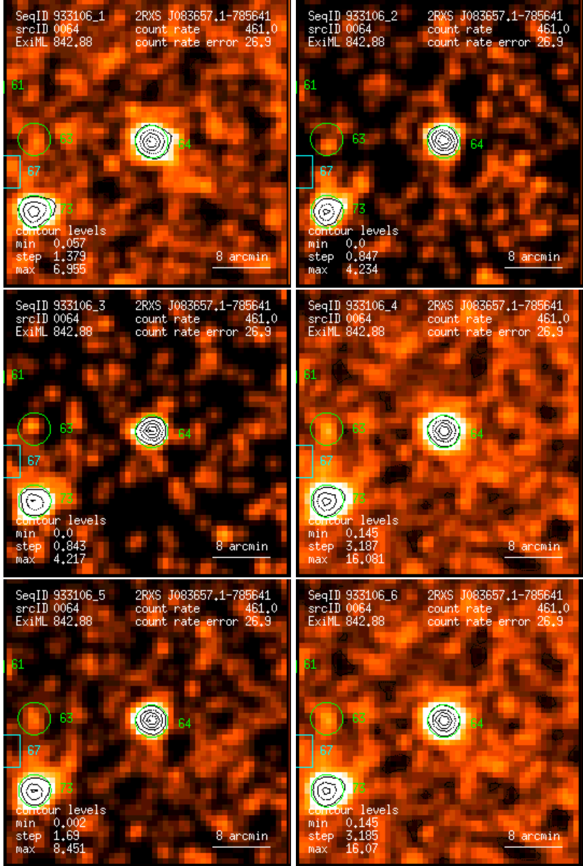
Figure 64: RASS 933106: detection 0064: band rate images, Gaussian filter: (1) PSPC channels 11 – 41, (2) 52 – 90, (3) 91 – 201, (4) 11 – 235, (5) 52 – 201, (6) 11 – 201. Broad band rates in counts/ks. Band rate contour levels in counts/ks/arcmin 2 .
