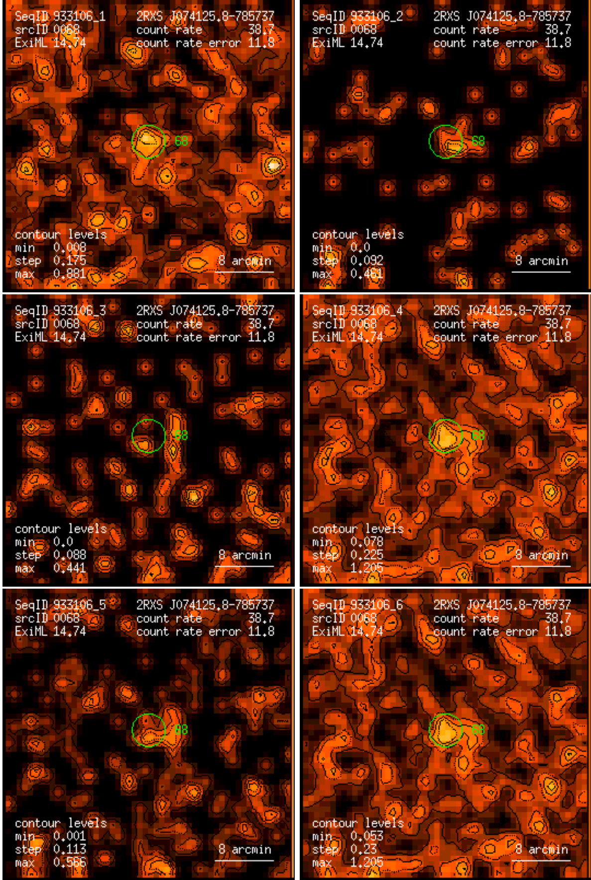
Figure 68: RASS 933106: detection 0068: band rate images, Gaussian filter: (1) PSPC channels 11 – 41, (2) 52 – 90, (3) 91 – 201, (4) 11 – 235, (5) 52 – 201, (6) 11 – 201. Broad band rates in counts/ks. Band rate contour levels in counts/ks/arcmin 2 .
