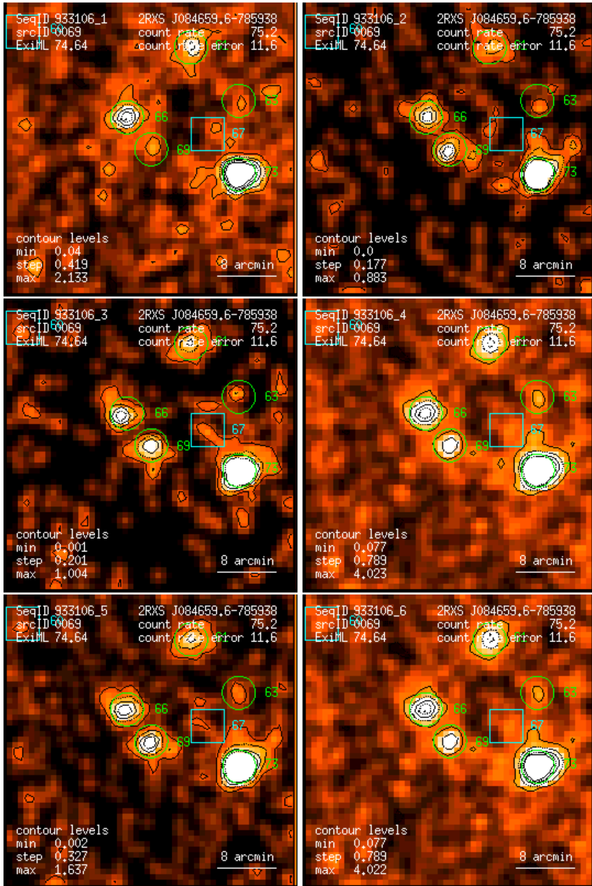
Figure 69: RASS 933106: detection 0069: band rate images, Gaussian filter: (1) PSPC channels 11 – 41, (2) 52 – 90, (3) 91 – 201, (4) 11 – 235, (5) 52 – 201, (6) 11 – 201. Broad band rates in counts/ks. Band rate contour levels in counts/ks/arcmin 2 .
