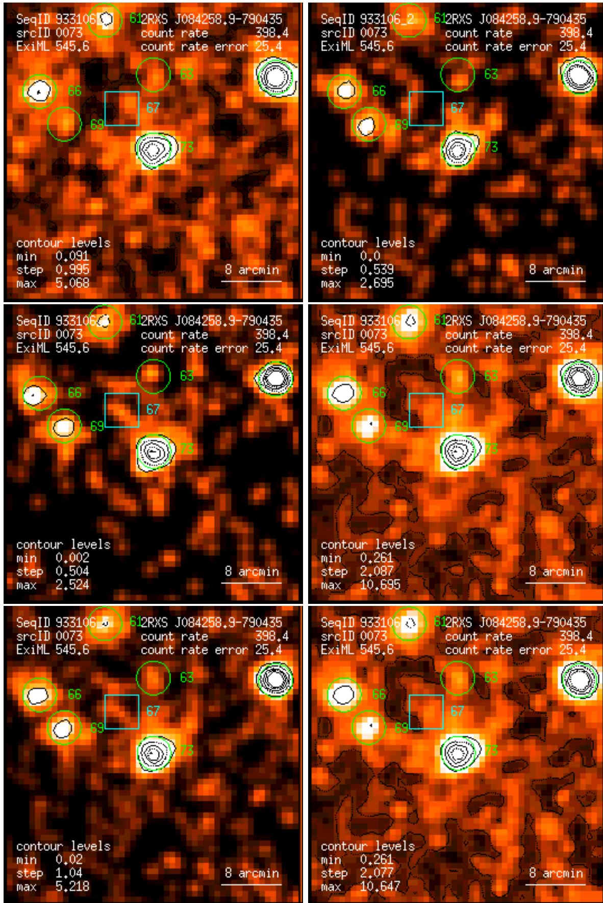
Figure 73: RASS 933106: detection 0073: band rate images, Gaussian filter: (1) PSPC channels 11 – 41, (2) 52 – 90, (3) 91 – 201, (4) 11 – 235, (5) 52 – 201, (6) 11 – 201. Broad band rates in counts/ks. Band rate contour levels in counts/ks/arcmin 2 .
