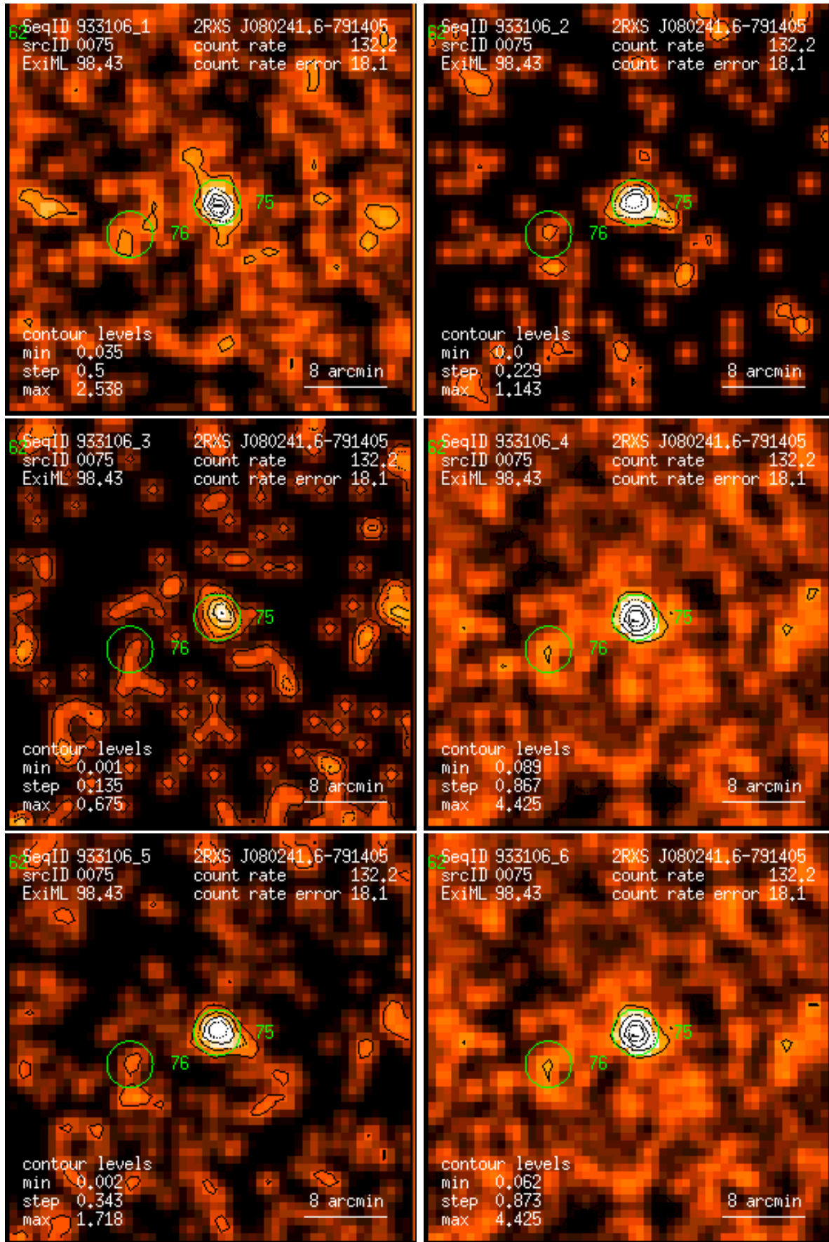
Figure 75: RASS 933106: detection 0075: band rate images, Gaussian filter: (1) PSPC channels 11 – 41, (2) 52 – 90, (3) 91 – 201, (4) 11 – 235, (5) 52 – 201, (6) 11 – 201. Broad band rates in counts/ks. Band rate contour levels in counts/ks/arcmin 2 .
