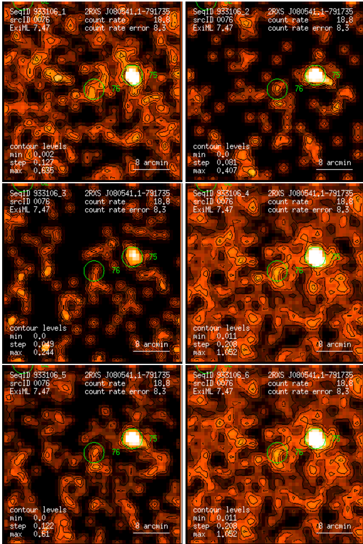
Figure 76: RASS 933106: detection 0076: band rate images, Gaussian filter: (1) PSPC channels 11 – 41, (2) 52 – 90, (3) 91 – 201, (4) 11 – 235, (5) 52 – 201, (6) 11 – 201. Broad band rates in counts/ks. Band rate contour levels in counts/ks/arcmin 2 .
