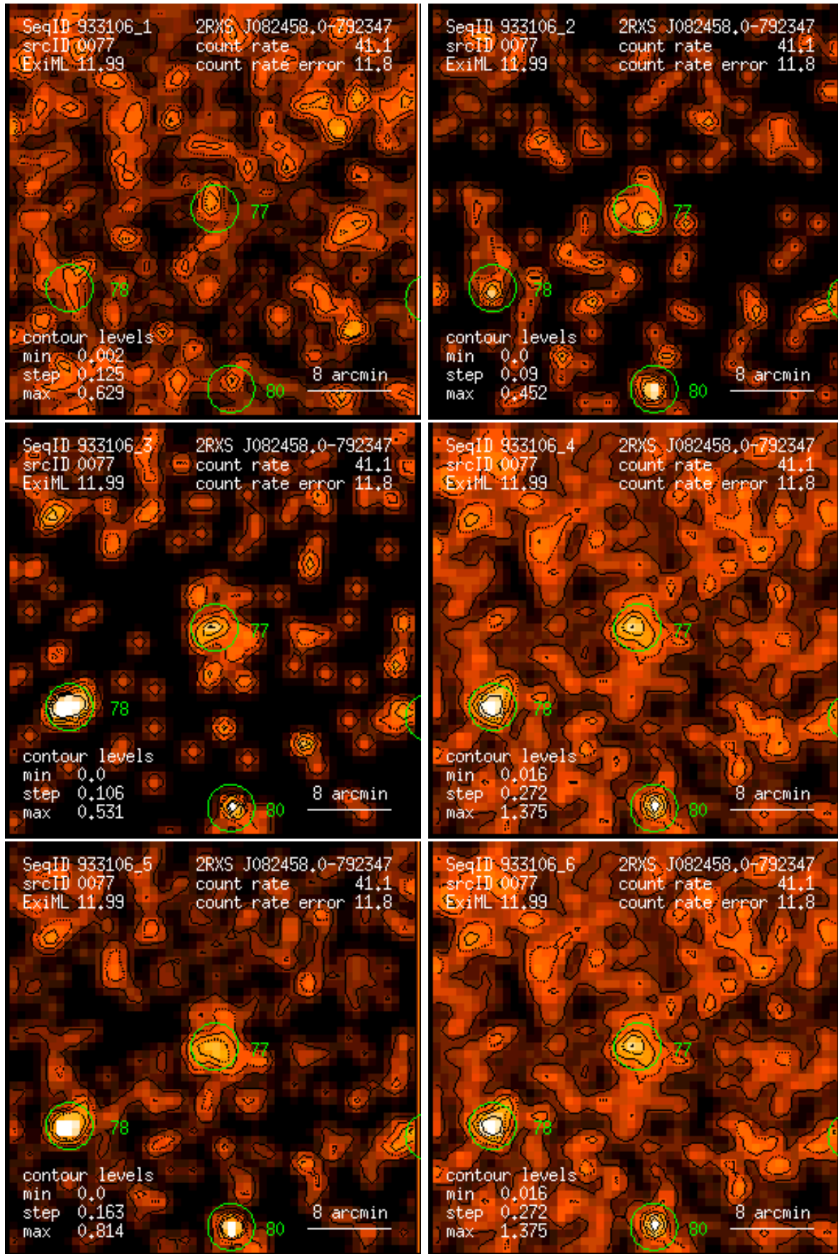
Figure 77: RASS 933106: detection 0077: band rate images, Gaussian filter: (1) PSPC channels 11 – 41, (2) 52 – 90, (3) 91 – 201, (4) 11 – 235, (5) 52 – 201, (6) 11 – 201. Broad band rates in counts/ks. Band rate contour levels in counts/ks/arcmin 2 .
