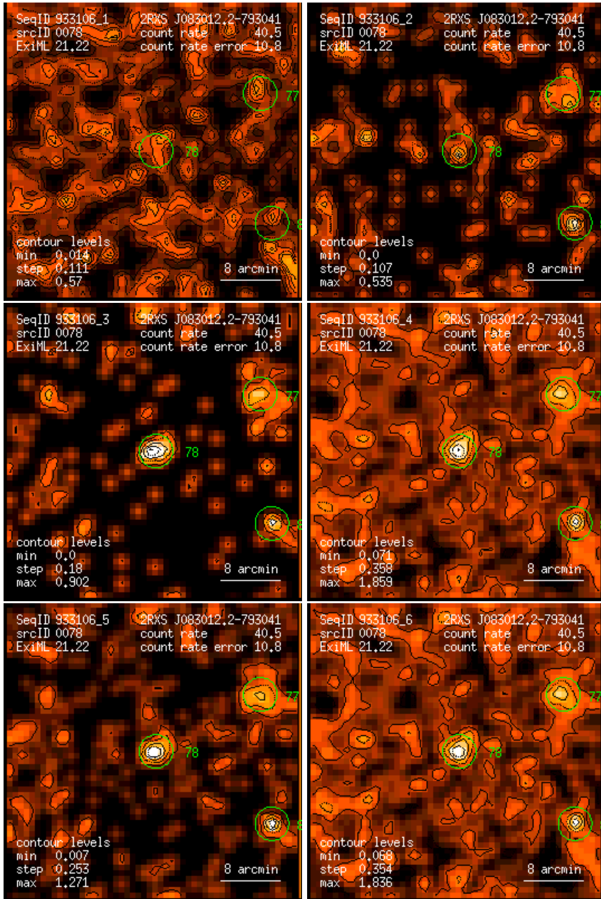
Figure 78: RASS 933106: detection 0078: band rate images, Gaussian filter: (1) PSPC channels 11 – 41, (2) 52 – 90, (3) 91 – 201, (4) 11 – 235, (5) 52 – 201, (6) 11 – 201. Broad band rates in counts/ks. Band rate contour levels in counts/ks/arcmin 2 .
