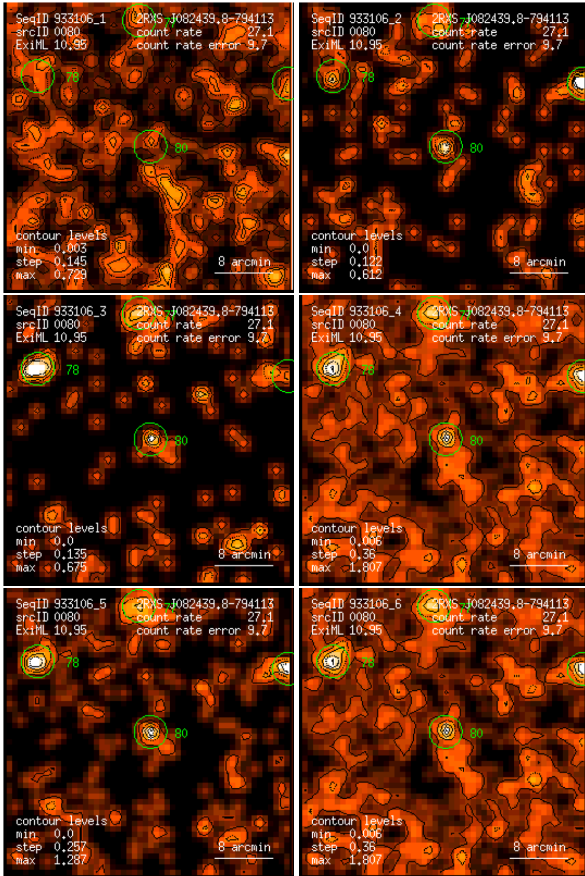
Figure 80: RASS 933106: detection 0080: band rate images, Gaussian filter: (1) PSPC channels 11 – 41, (2) 52 – 90, (3) 91 – 201, (4) 11 – 235, (5) 52 – 201, (6) 11 – 201. Broad band rates in counts/ks. Band rate contour levels in counts/ks/arcmin 2 .
