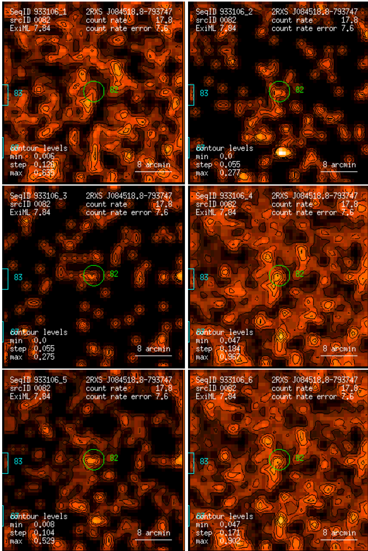
Figure 82: RASS 933106: detection 0082: band rate images, Gaussian filter: (1) PSPC channels 11 – 41, (2) 52 – 90, (3) 91 – 201, (4) 11 – 235, (5) 52 – 201, (6) 11 – 201. Broad band rates in counts/ks. Band rate contour levels in counts/ks/arcmin 2 .
