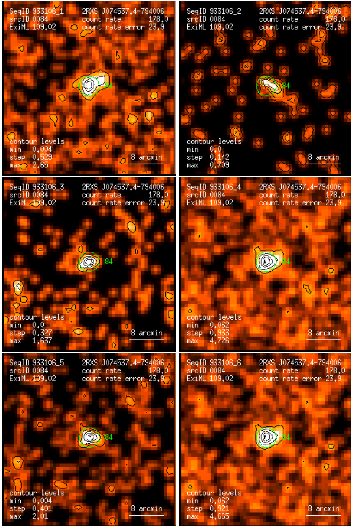
Figure 84: RASS 933106: detection 0084: band rate images, Gaussian filter: (1) PSPC channels 11 – 41, (2) 52 – 90, (3) 91 – 201, (4) 11 – 235, (5) 52 – 201, (6) 11 – 201. Broad band rates in counts/ks. Band rate contour levels in counts/ks/arcmin 2 .
