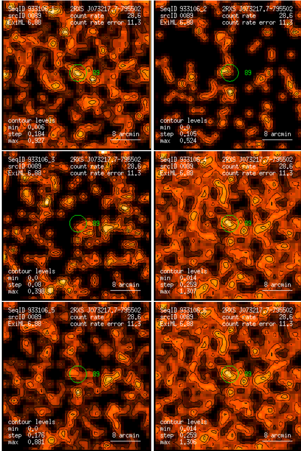
Figure 89: RASS 933106: detection 0089: band rate images, Gaussian filter: (1) PSPC channels 11 – 41, (2) 52 – 90, (3) 91 – 201, (4) 11 – 235, (5) 52 – 201, (6) 11 – 201. Broad band rates in counts/ks. Band rate contour levels in counts/ks/arcmin 2 .
