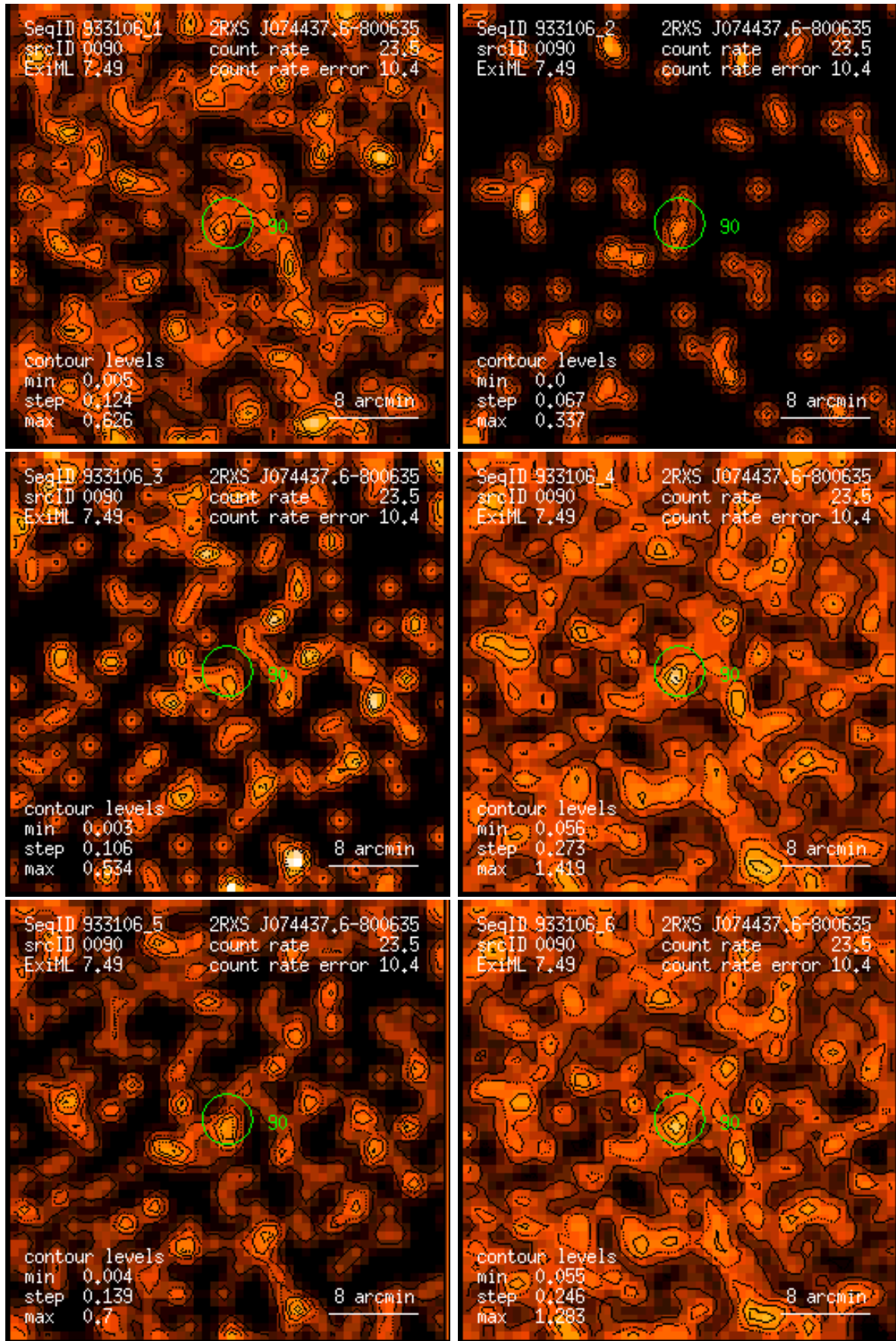
Figure 90: RASS 933106: detection 0090: band rate images, Gaussian filter: (1) PSPC channels 11 – 41, (2) 52 – 90, (3) 91 – 201, (4) 11 – 235, (5) 52 – 201, (6) 11 – 201. Broad band rates in counts/ks. Band rate contour levels in counts/ks/arcmin 2 .
