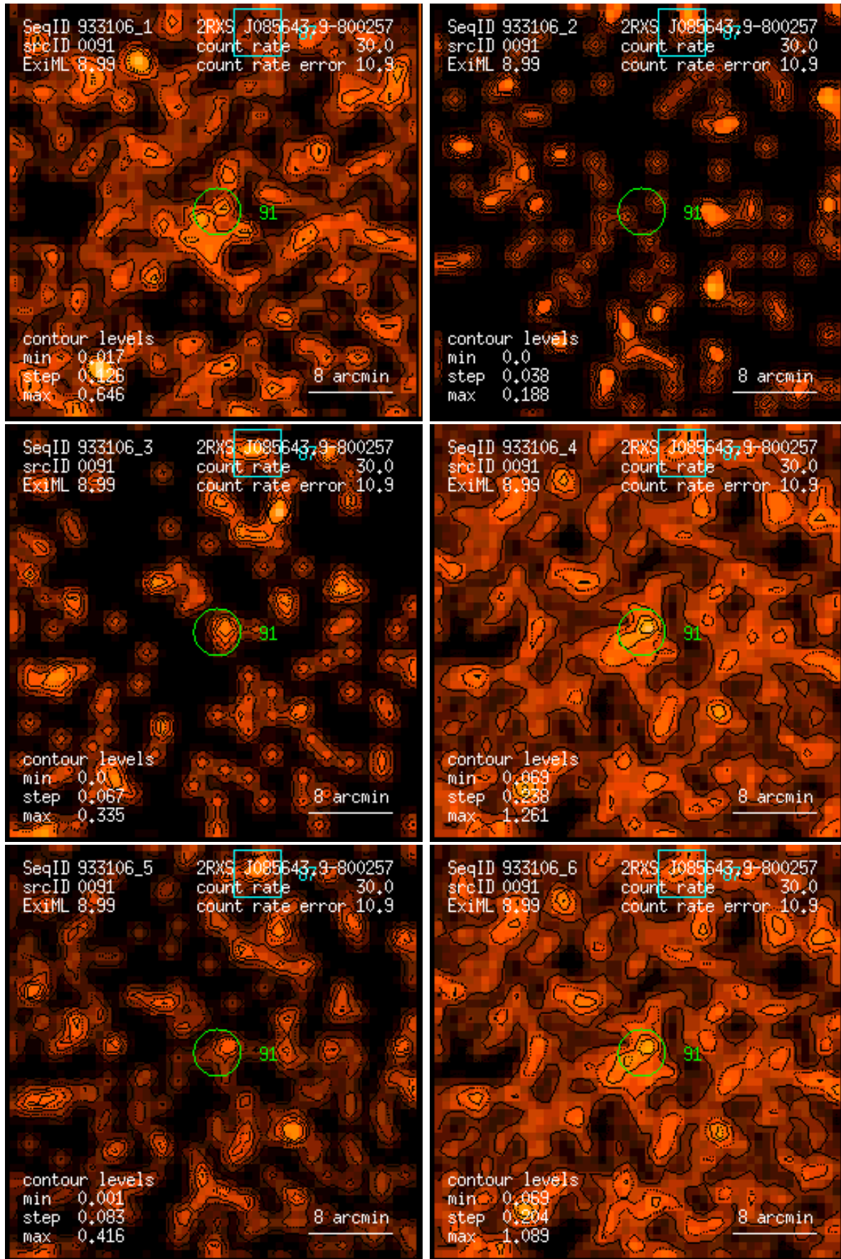
Figure 91: RASS 933106: detection 0091: band rate images, Gaussian filter: (1) PSPC channels 11 – 41, (2) 52 – 90, (3) 91 – 201, (4) 11 – 235, (5) 52 – 201, (6) 11 – 201. Broad band rates in counts/ks. Band rate contour levels in counts/ks/arcmin 2 .
