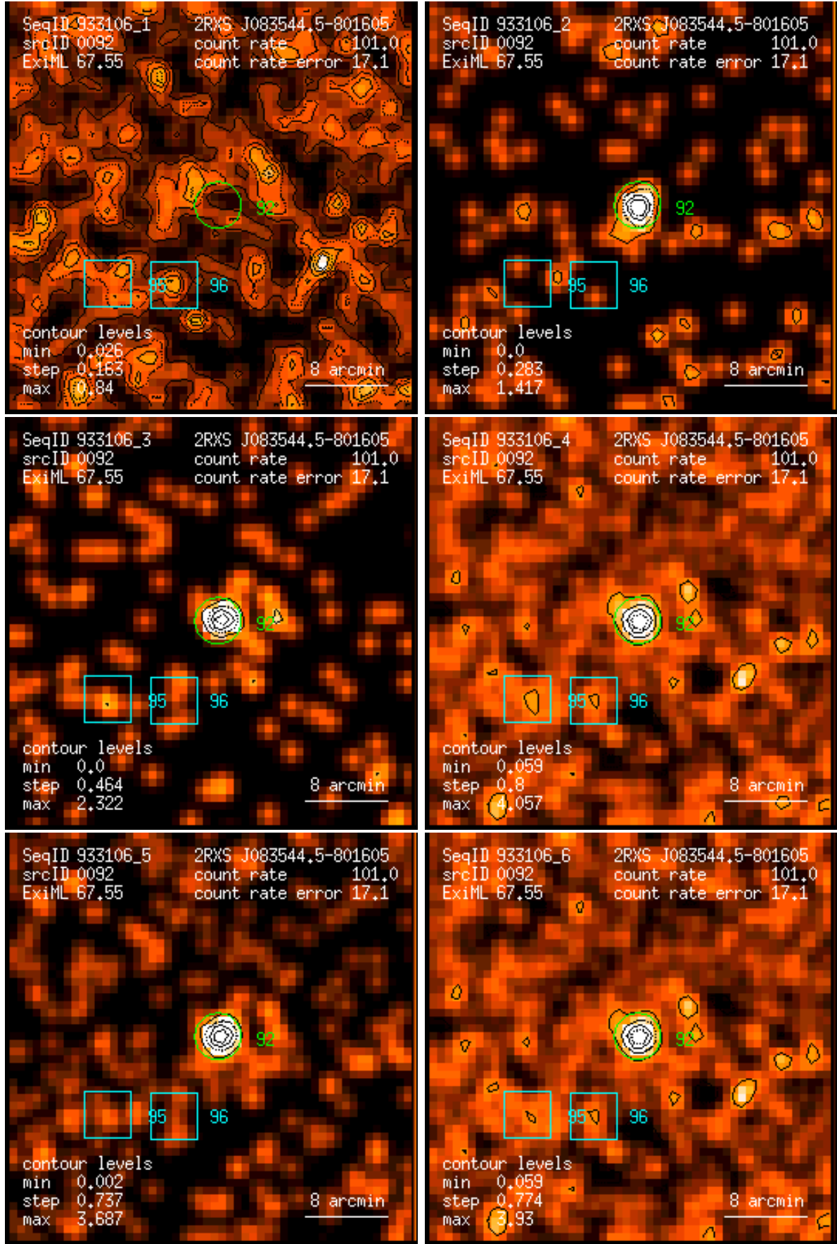
Figure 92: RASS 933106: detection 0092: band rate images, Gaussian filter: (1) PSPC channels 11 – 41, (2) 52 – 90, (3) 91 – 201, (4) 11 – 235, (5) 52 – 201, (6) 11 – 201. Broad band rates in counts/ks. Band rate contour levels in counts/ks/arcmin 2 .
