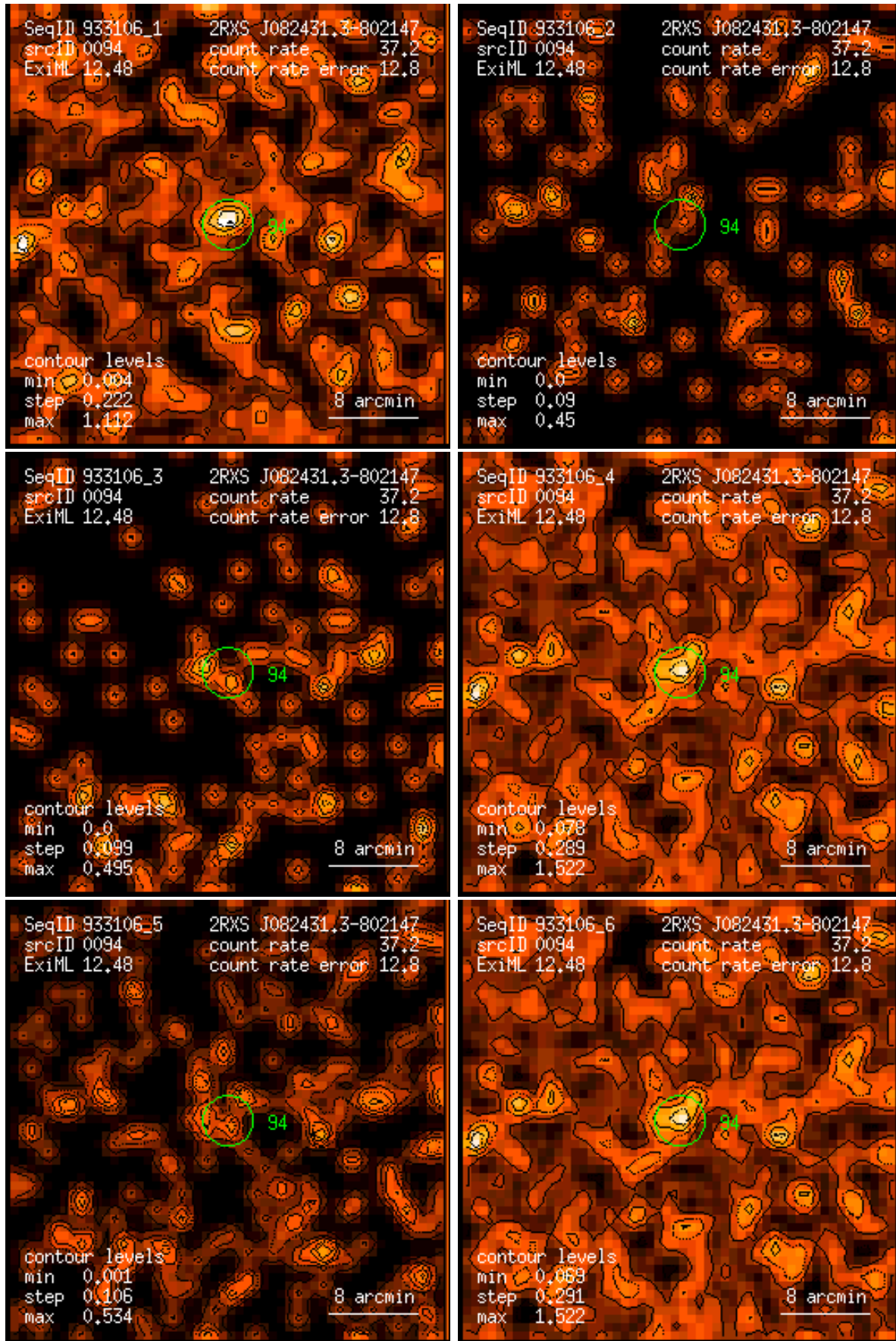
Figure 94: RASS 933106: detection 0094: band rate images, Gaussian filter: (1) PSPC channels 11 – 41, (2) 52 – 90, (3) 91 – 201, (4) 11 – 235, (5) 52 – 201, (6) 11 – 201. Broad band rates in counts/ks. Band rate contour levels in counts/ks/arcmin 2 .
