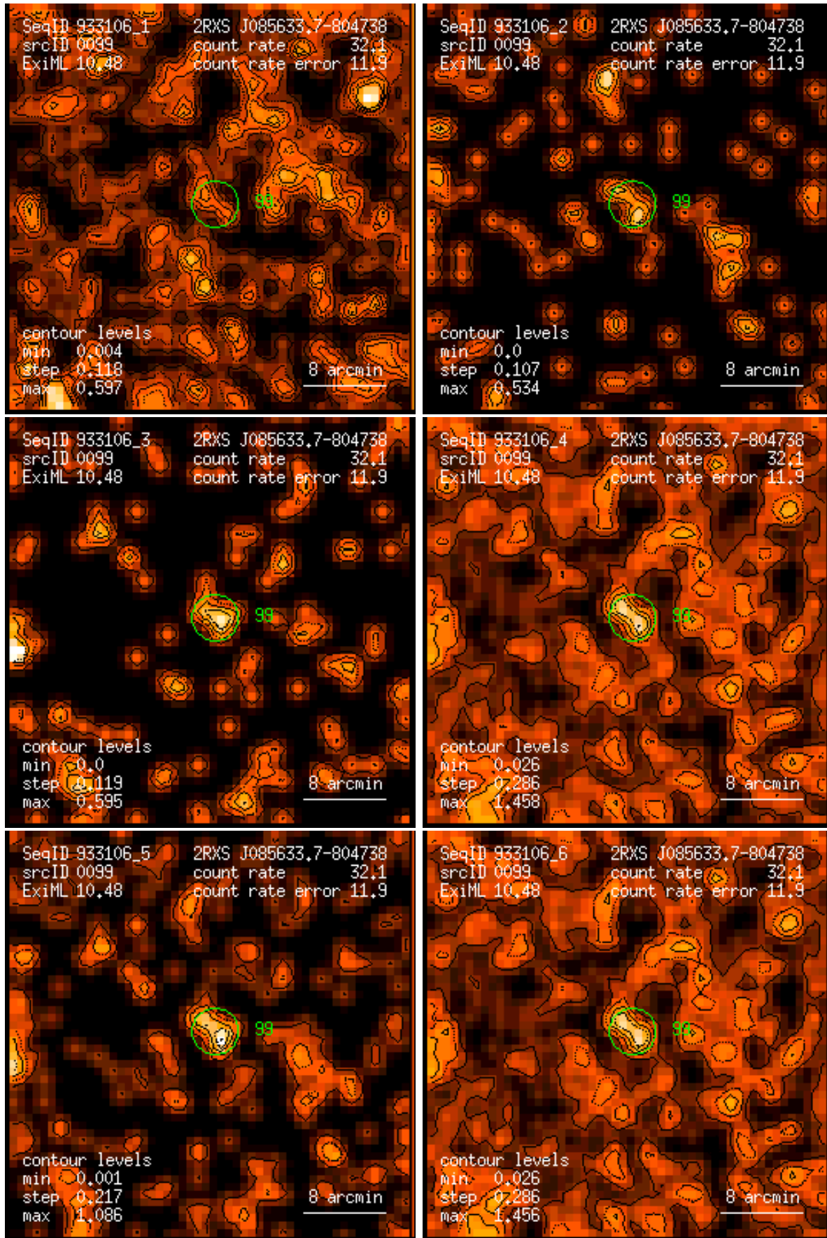
Figure 99: RASS 933106: detection 0099: band rate images, Gaussian filter: (1) PSPC channels 11 – 41, (2) 52 – 90, (3) 91 – 201, (4) 11 – 235, (5) 52 – 201, (6) 11 – 201. Broad band rates in counts/ks. Band rate contour levels in counts/ks/arcmin 2 .
