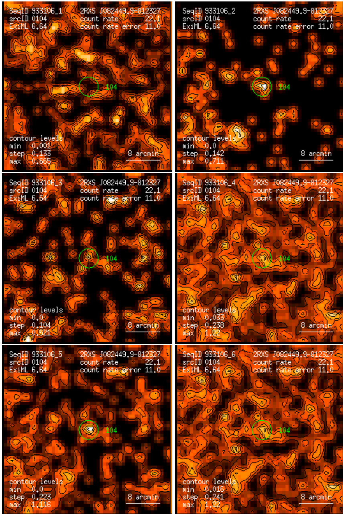
Figure 104: RASS 933106: detection 0104: band rate images, Gaussian filter: (1) PSPC channels 11 – 41, (2) 52 – 90, (3) 91 – 201, (4) 11 – 235, (5) 52 – 201, (6) 11 – 201. Broad band rates in counts/ks. Band rate contour levels in counts/ks/arcmin 2 .
