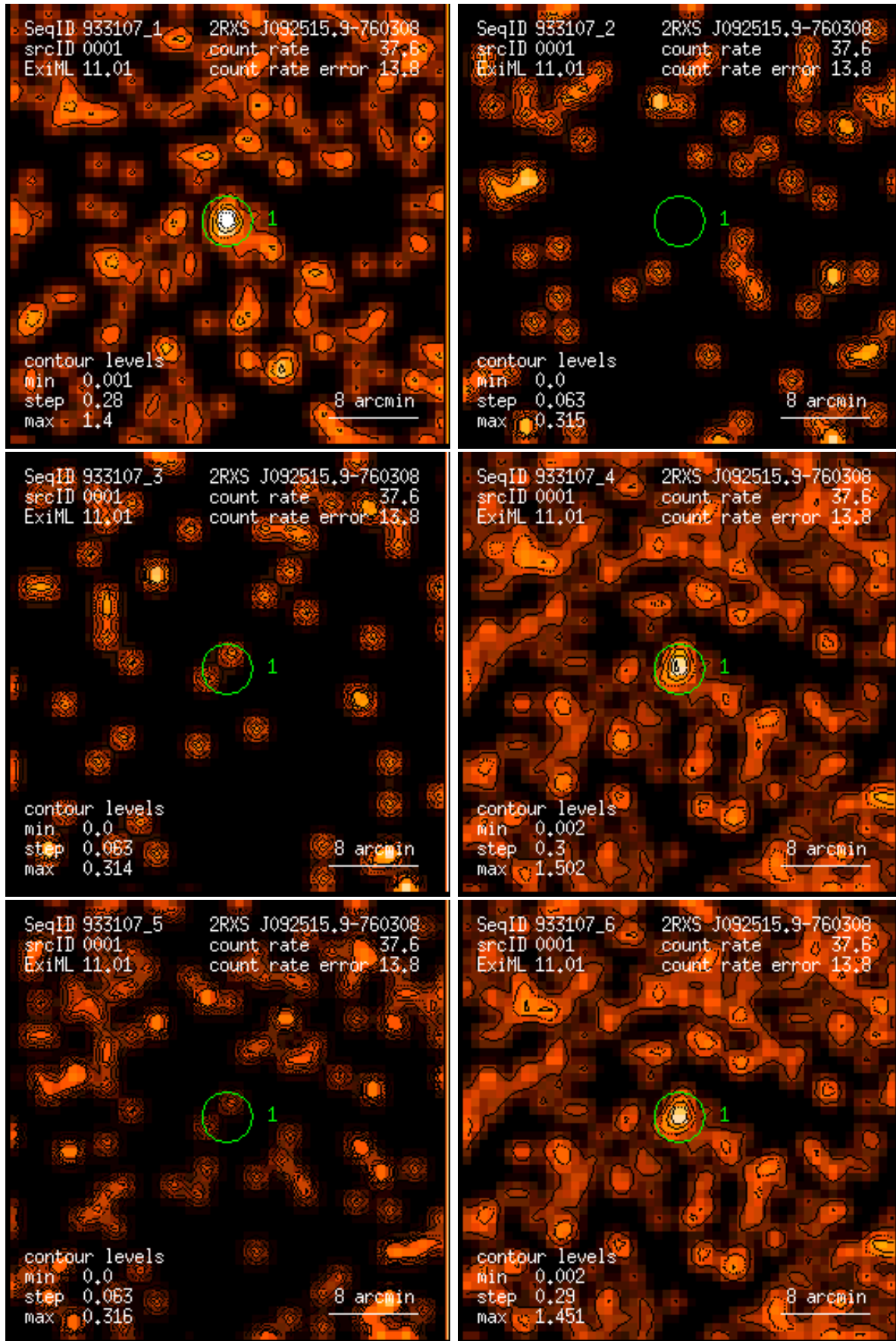
Figure 1: RASS 933107: detection 0001: band rate images, Gaussian filter: (1) PSPC channels 11 – 41, (2) 52 – 90, (3) 91 – 201, (4) 11 – 235, (5) 52 – 201, (6) 11 – 201. Broad band rates in counts/ks. Band rate contour levels in counts/ks/arcmin 2 .
