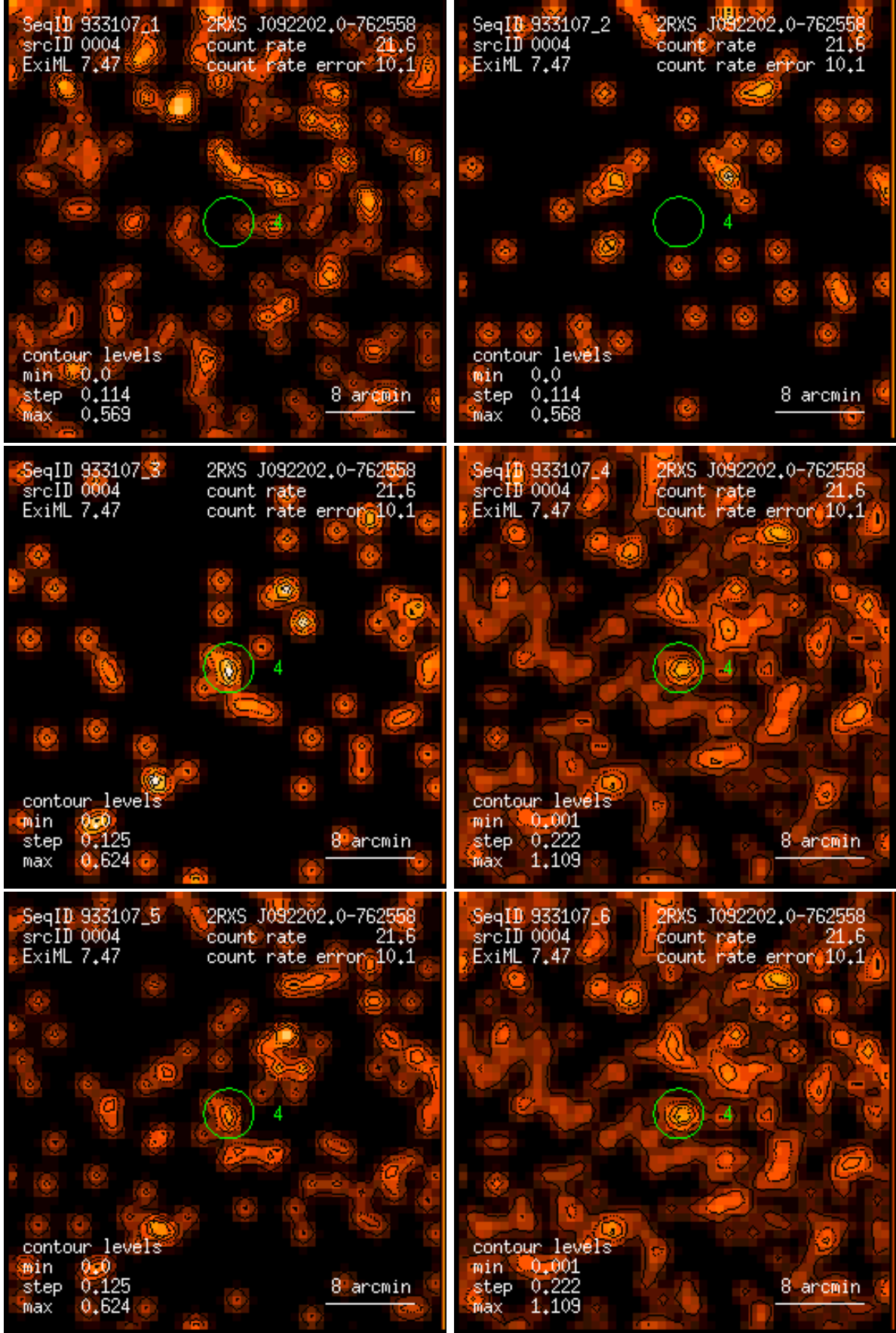
Figure 4: RASS 933107: detection 0004: band rate images, Gaussian filter: (1) PSPC channels 11 – 41, (2) 52 – 90, (3) 91 – 201, (4) 11 – 235, (5) 52 – 201, (6) 11 – 201. Broad band rates in counts/ks. Band rate contour levels in counts/ks/arcmin 2 .
