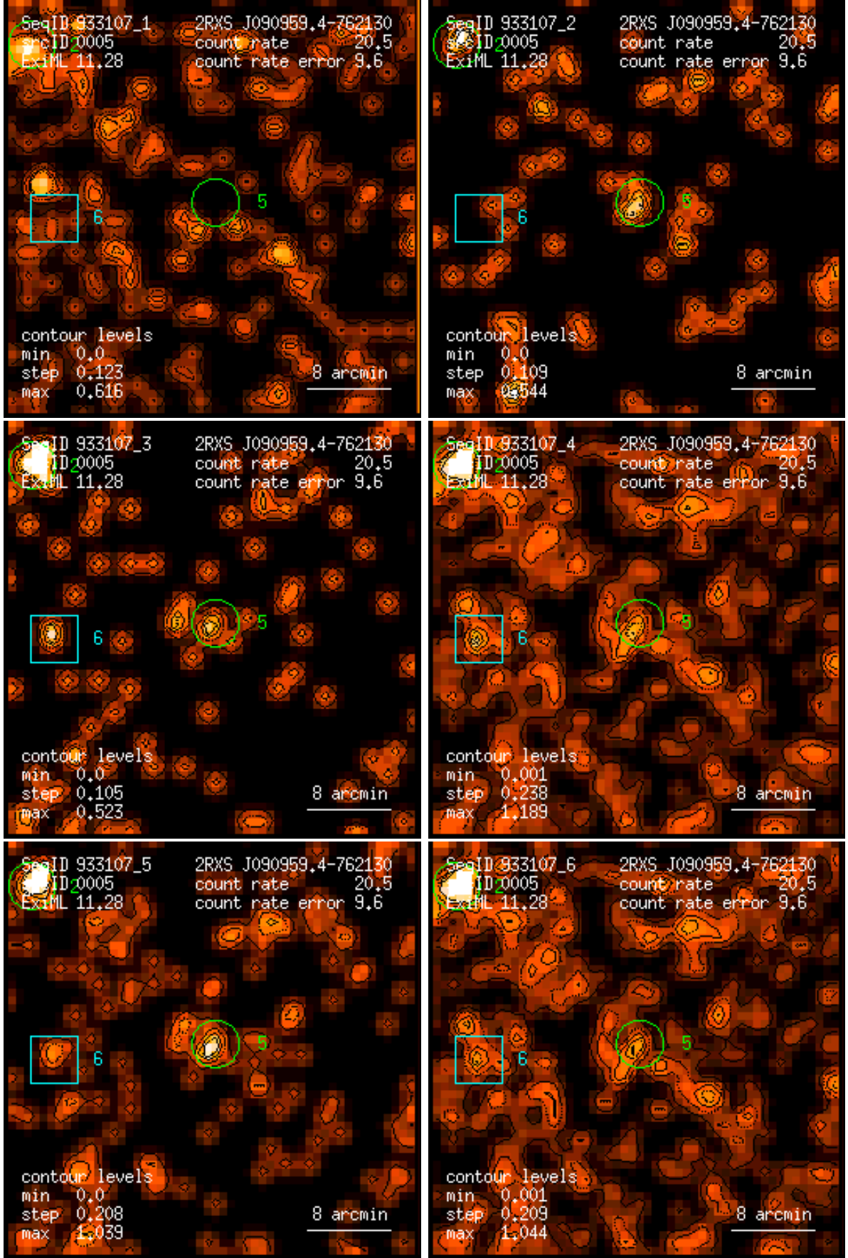
Figure 5: RASS 933107: detection 0005: band rate images, Gaussian filter: (1) PSPC channels 11 – 41, (2) 52 – 90, (3) 91 – 201, (4) 11 – 235, (5) 52 – 201, (6) 11 – 201. Broad band rates in counts/ks. Band rate contour levels in counts/ks/arcmin 2 .
