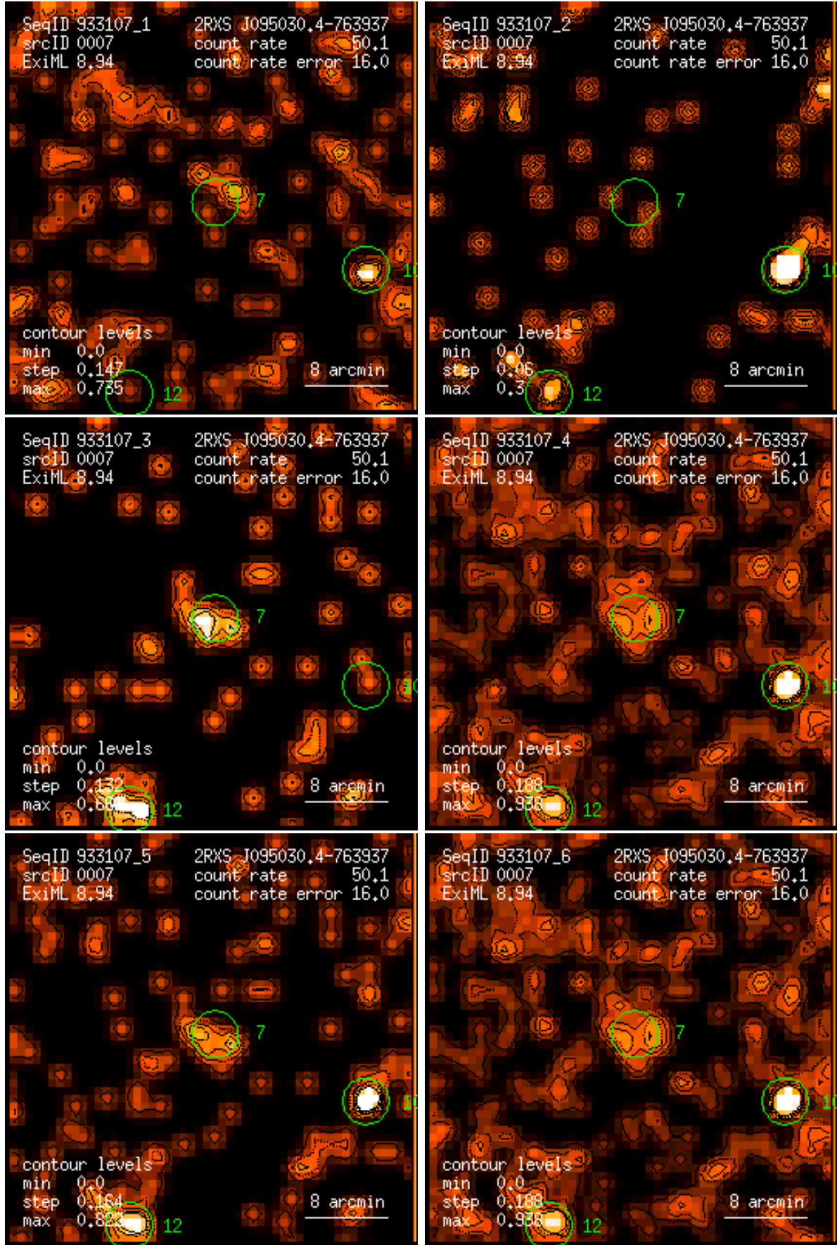
Figure 7: RASS 933107: detection 0007: band rate images, Gaussian filter: (1) PSPC channels 11 – 41, (2) 52 – 90, (3) 91 – 201, (4) 11 – 235, (5) 52 – 201, (6) 11 – 201. Broad band rates in counts/ks. Band rate contour levels in counts/ks/arcmin 2 .
