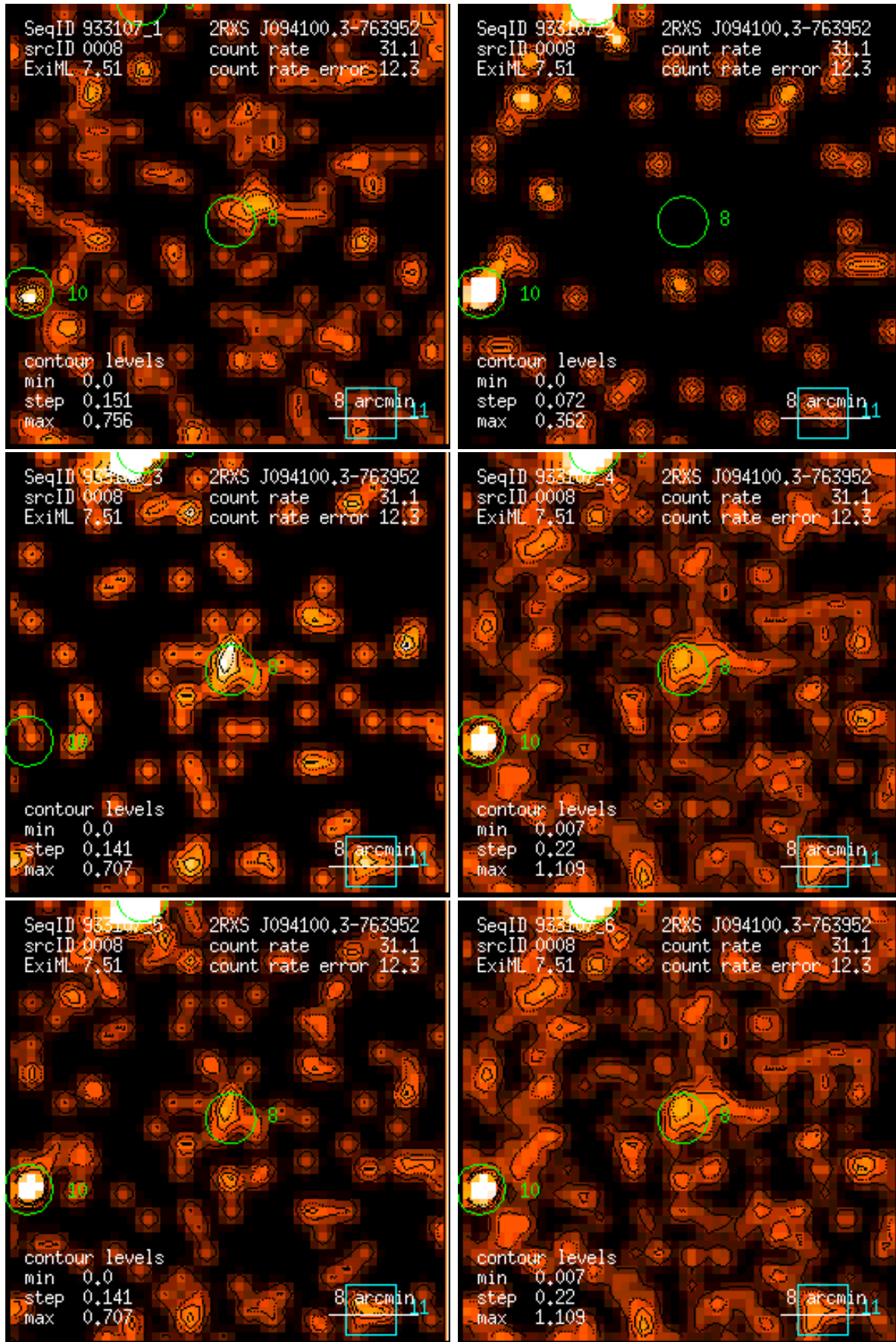
Figure 8: RASS 933107: detection 0008: band rate images, Gaussian filter: (1) PSPC channels 11 – 41, (2) 52 – 90, (3) 91 – 201, (4) 11 – 235, (5) 52 – 201, (6) 11 – 201. Broad band rates in counts/ks. Band rate contour levels in counts/ks/arcmin 2 .
