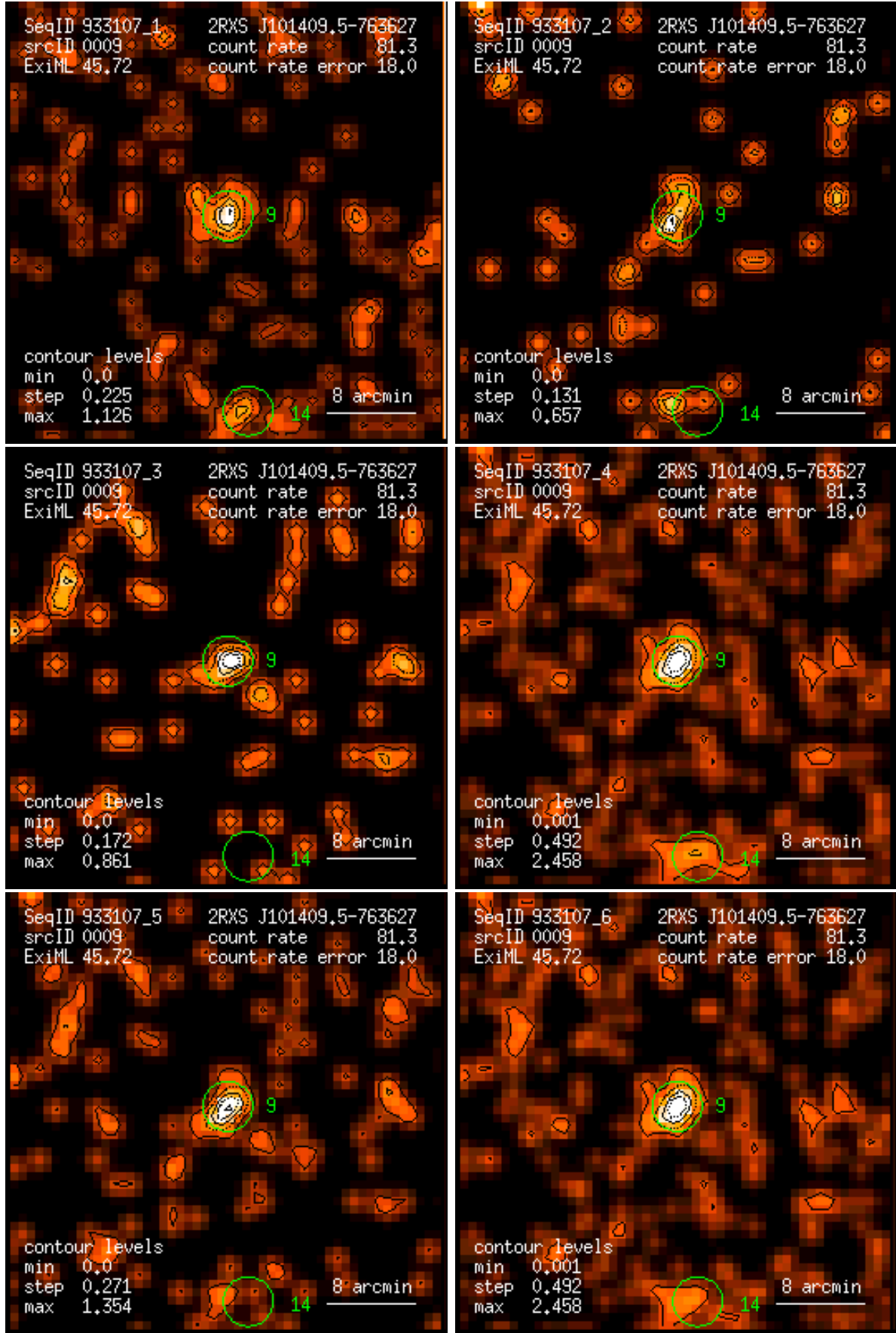
Figure 9: RASS 933107: detection 0009: band rate images, Gaussian filter: (1) PSPC channels 11 – 41, (2) 52 – 90, (3) 91 – 201, (4) 11 – 235, (5) 52 – 201, (6) 11 – 201. Broad band rates in counts/ks. Band rate contour levels in counts/ks/arcmin 2 .
