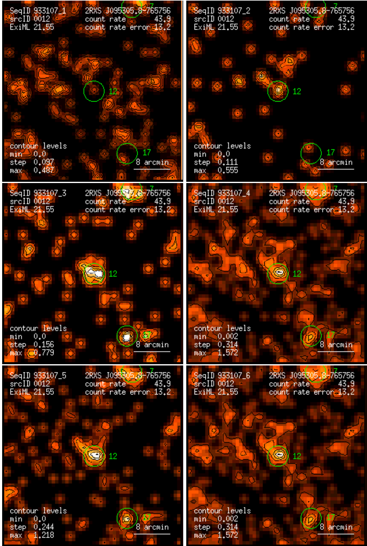
Figure 12: RASS 933107: detection 0012: band rate images, Gaussian filter: (1) PSPC channels 11 – 41, (2) 52 – 90, (3) 91 – 201, (4) 11 – 235, (5) 52 – 201, (6) 11 – 201. Broad band rates in counts/ks. Band rate contour levels in counts/ks/arcmin 2 .
