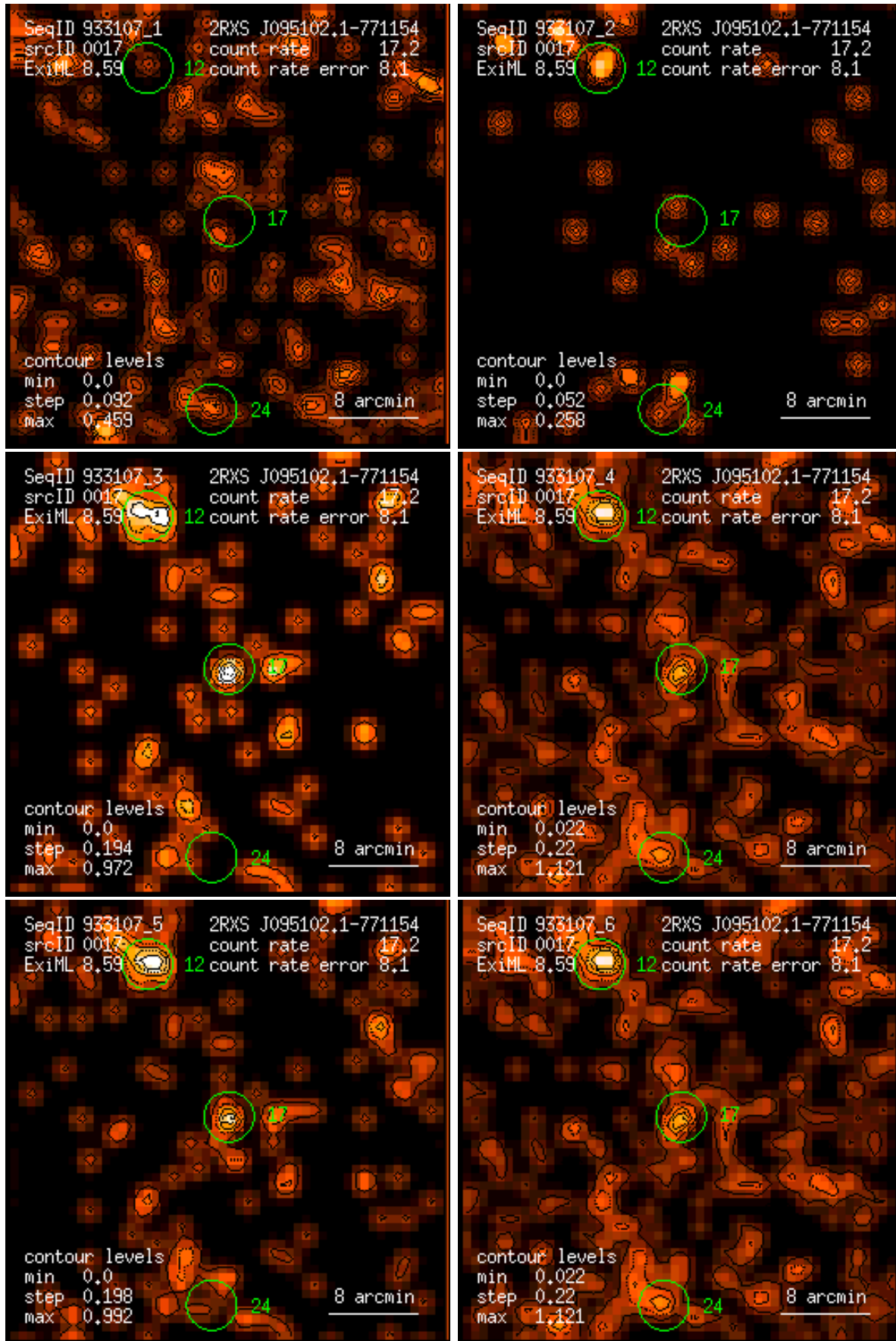
Figure 17: RASS 933107: detection 0017: band rate images, Gaussian filter: (1) PSPC channels 11 – 41, (2) 52 – 90, (3) 91 – 201, (4) 11 – 235, (5) 52 – 201, (6) 11 – 201. Broad band rates in counts/ks. Band rate contour levels in counts/ks/arcmin 2 .
