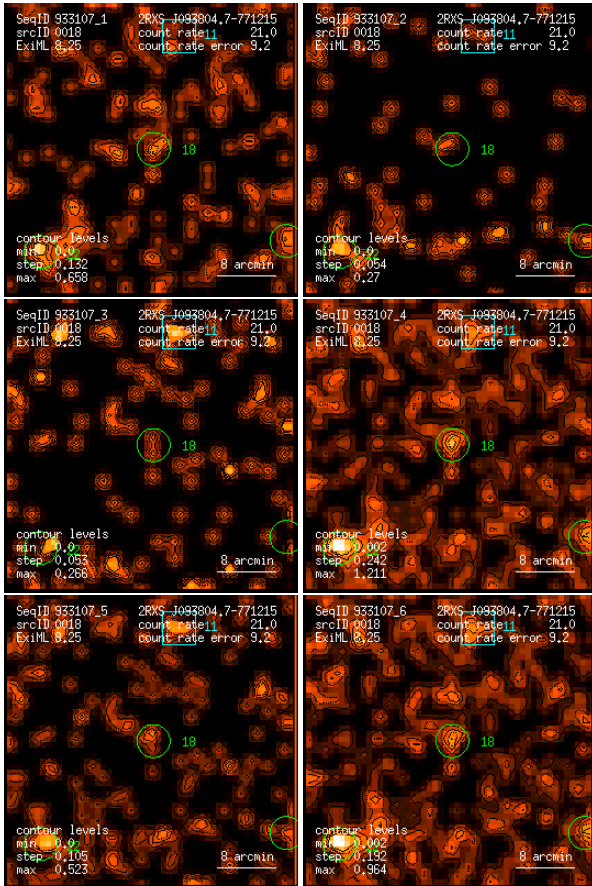
Figure 18: RASS 933107: detection 0018: band rate images, Gaussian filter: (1) PSPC channels 11 – 41, (2) 52 – 90, (3) 91 – 201, (4) 11 – 235, (5) 52 – 201, (6) 11 – 201. Broad band rates in counts/ks. Band rate contour levels in counts/ks/arcmin 2 .
