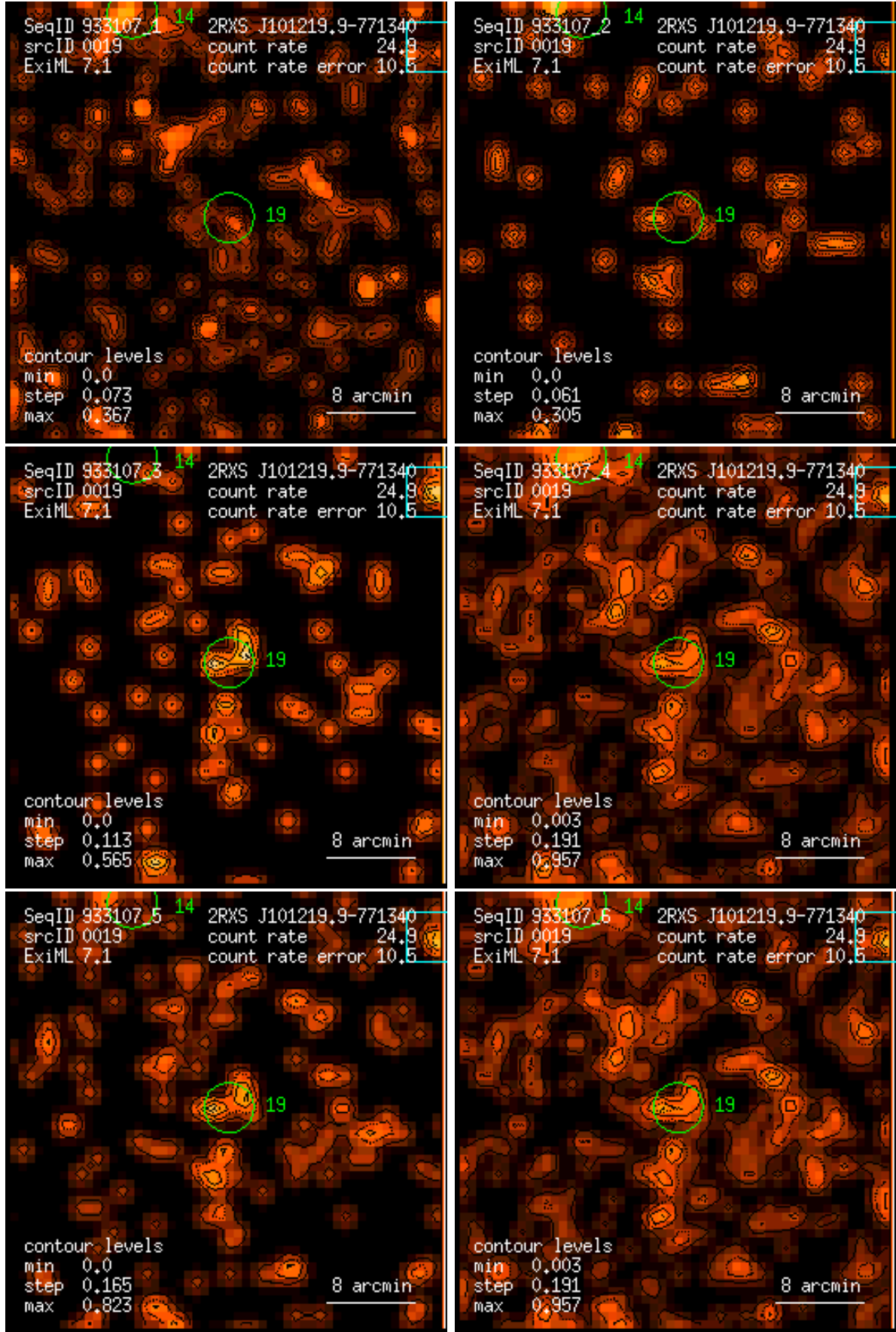
Figure 19: RASS 933107: detection 0019: band rate images, Gaussian filter: (1) PSPC channels 11 – 41, (2) 52 – 90, (3) 91 – 201, (4) 11 – 235, (5) 52 – 201, (6) 11 – 201. Broad band rates in counts/ks. Band rate contour levels in counts/ks/arcmin 2 .
