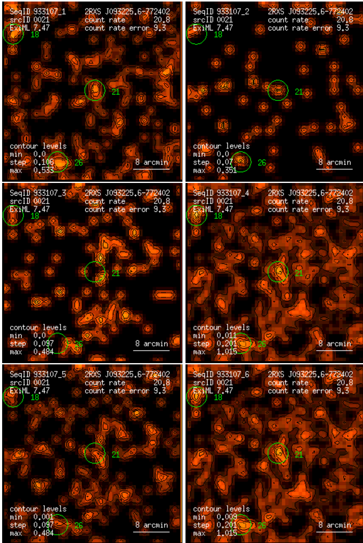
Figure 21: RASS 933107: detection 0021: band rate images, Gaussian filter: (1) PSPC channels 11 – 41, (2) 52 – 90, (3) 91 – 201, (4) 11 – 235, (5) 52 – 201, (6) 11 – 201. Broad band rates in counts/ks. Band rate contour levels in counts/ks/arcmin 2 .
