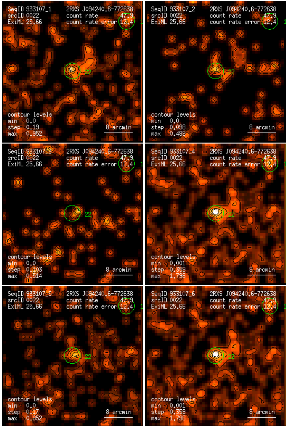
Figure 22: RASS 933107: detection 0022: band rate images, Gaussian filter: (1) PSPC channels 11 – 41, (2) 52 – 90, (3) 91 – 201, (4) 11 – 235, (5) 52 – 201, (6) 11 – 201. Broad band rates in counts/ks. Band rate contour levels in counts/ks/arcmin 2 .
