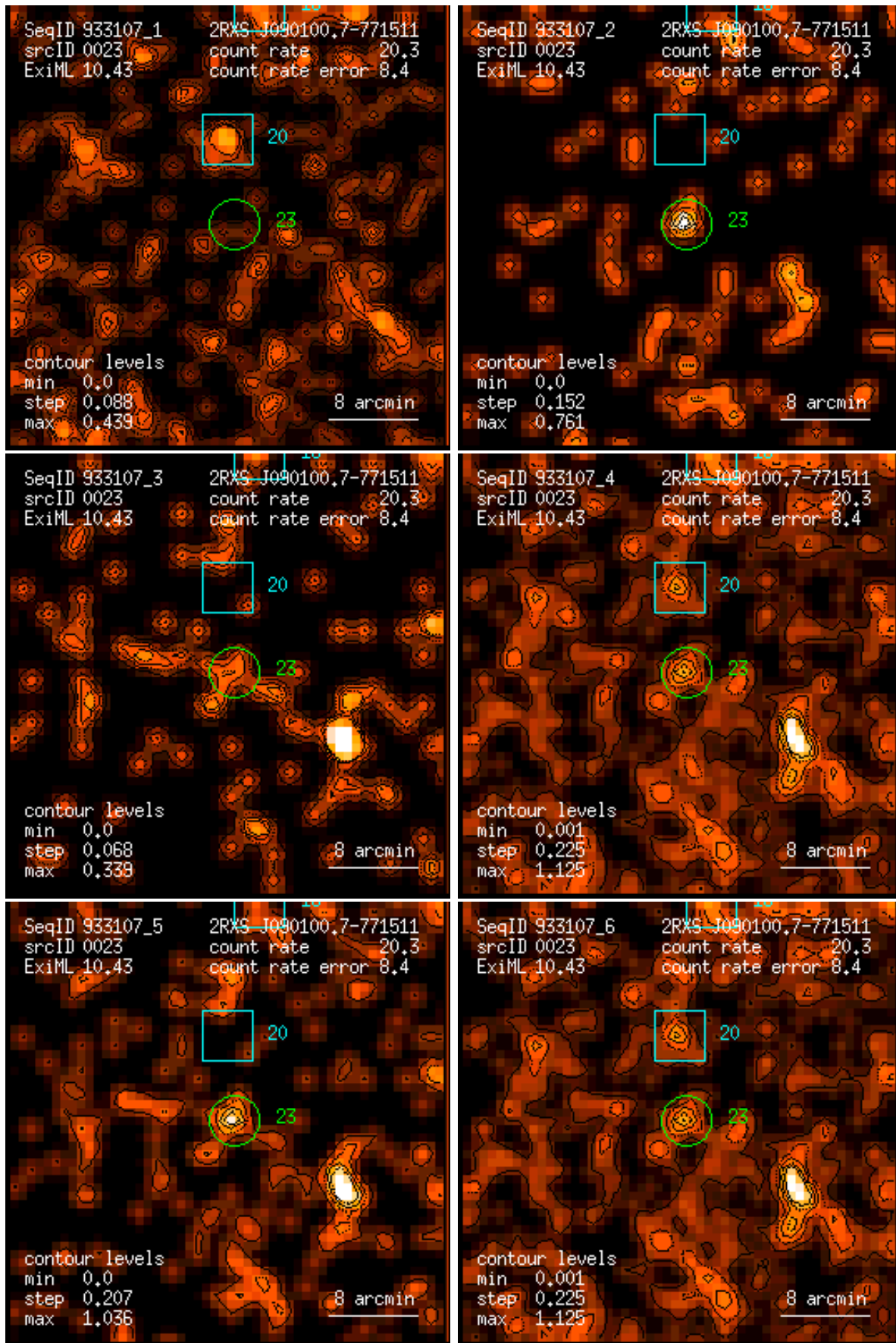
Figure 23: RASS 933107: detection 0023: band rate images, Gaussian filter: (1) PSPC channels 11 – 41, (2) 52 – 90, (3) 91 – 201, (4) 11 – 235, (5) 52 – 201, (6) 11 – 201. Broad band rates in counts/ks. Band rate contour levels in counts/ks/arcmin 2 .
