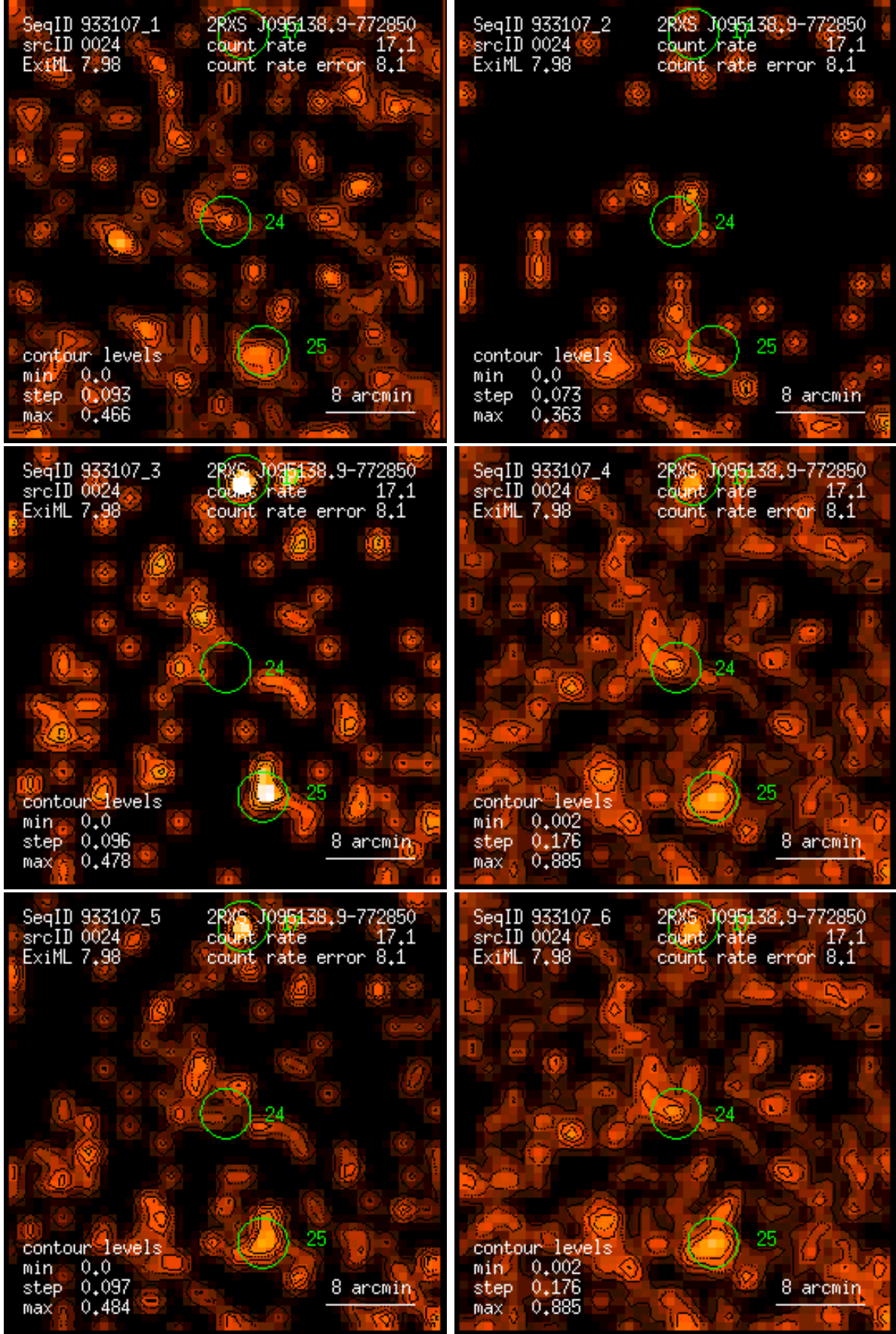
Figure 24: RASS 933107: detection 0024: band rate images, Gaussian filter: (1) PSPC channels 11 – 41, (2) 52 – 90, (3) 91 – 201, (4) 11 – 235, (5) 52 – 201, (6) 11 – 201. Broad band rates in counts/ks. Band rate contour levels in counts/ks/arcmin 2 .
