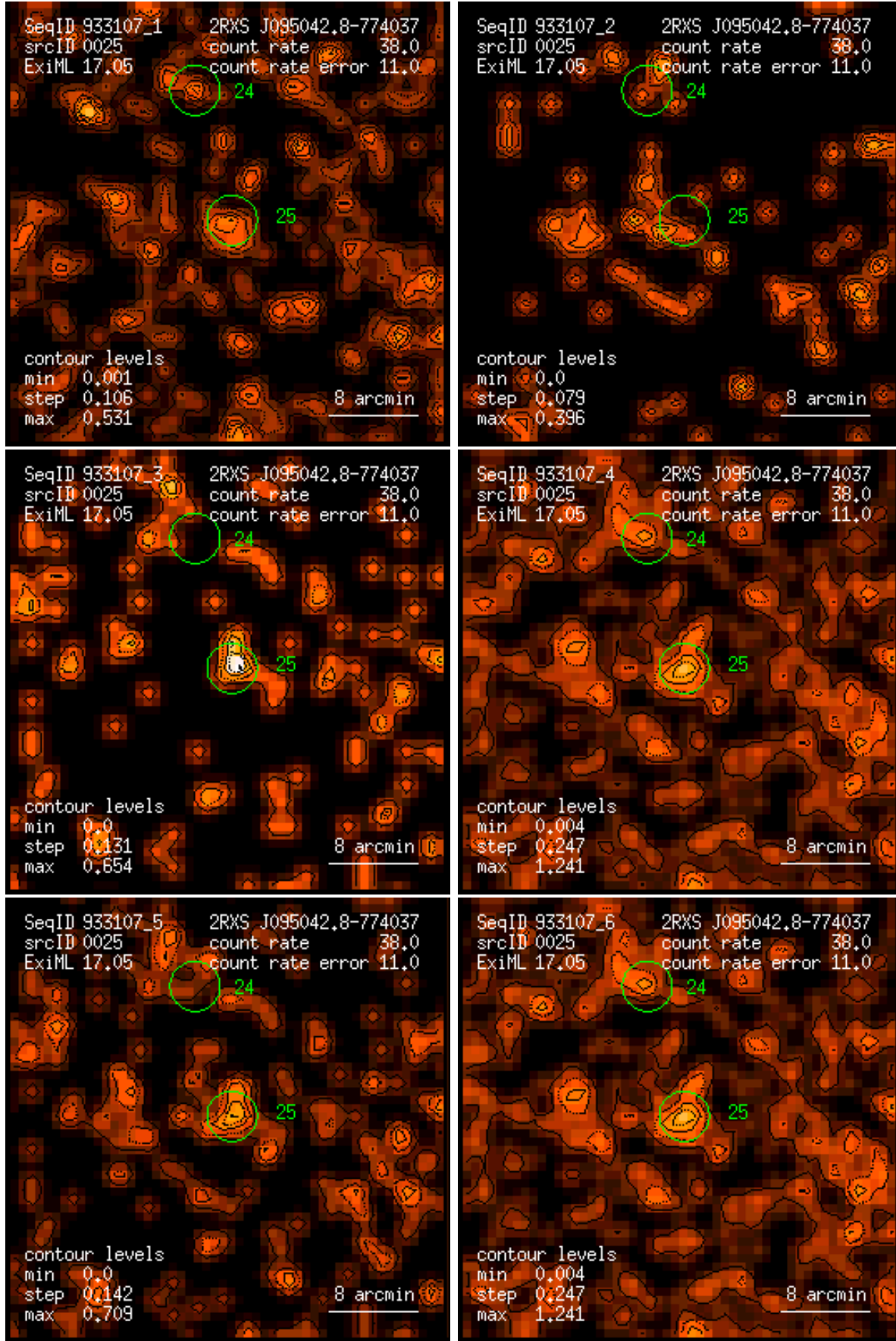
Figure 25: RASS 933107: detection 0025: band rate images, Gaussian filter: (1) PSPC channels 11 – 41, (2) 52 – 90, (3) 91 – 201, (4) 11 – 235, (5) 52 – 201, (6) 11 – 201. Broad band rates in counts/ks. Band rate contour levels in counts/ks/arcmin 2 .
