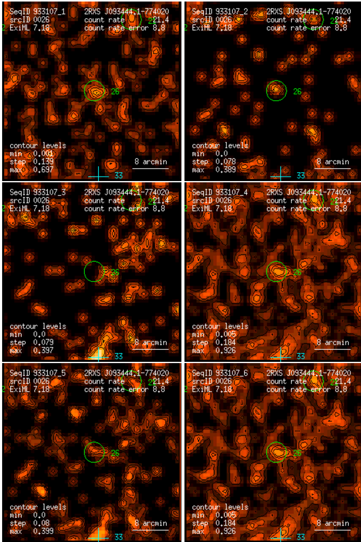
Figure 26: RASS 933107: detection 0026: band rate images, Gaussian filter: (1) PSPC channels 11 – 41, (2) 52 – 90, (3) 91 – 201, (4) 11 – 235, (5) 52 – 201, (6) 11 – 201. Broad band rates in counts/ks. Band rate contour levels in counts/ks/arcmin 2 .
