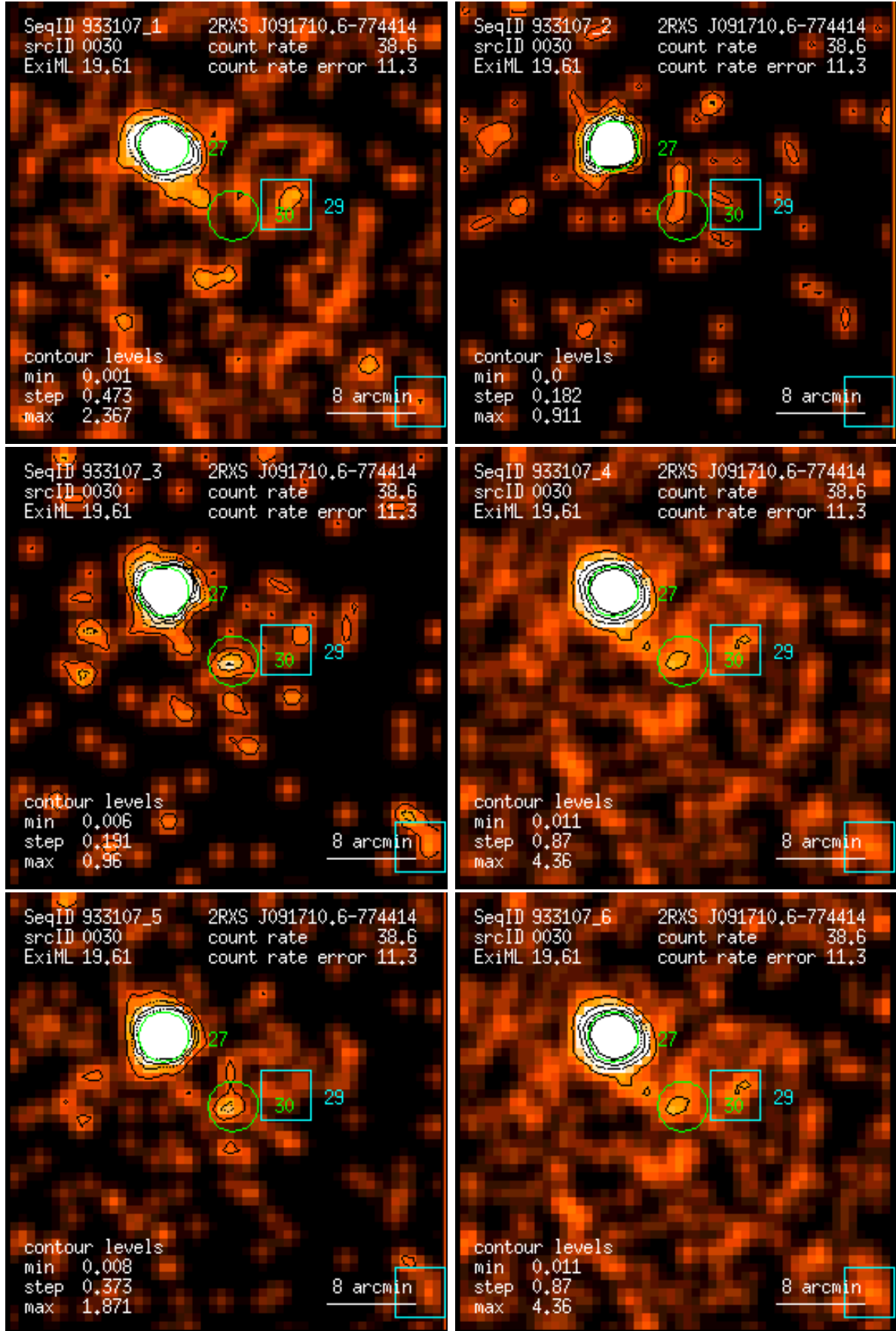
Figure 30: RASS 933107: detection 0030: band rate images, Gaussian filter: (1) PSPC channels 11 – 41, (2) 52 – 90, (3) 91 – 201, (4) 11 – 235, (5) 52 – 201, (6) 11 – 201. Broad band rates in counts/ks. Band rate contour levels in counts/ks/arcmin 2 .
